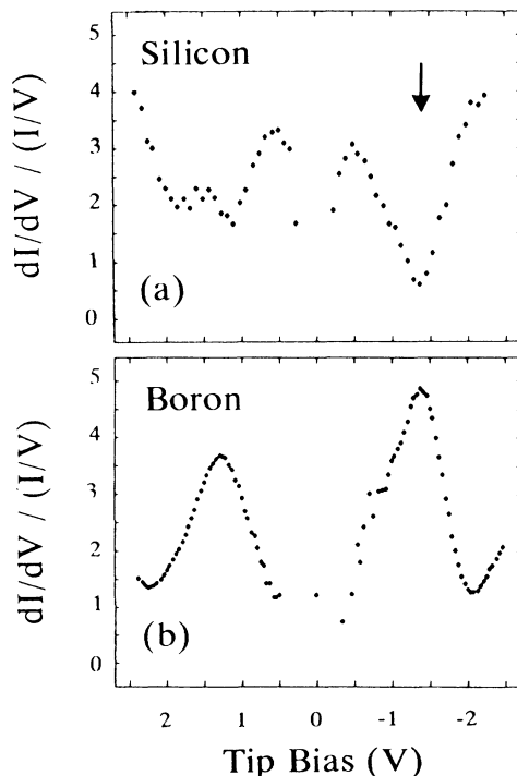
FIG. 2. Normalized differential conductivity spectra recorded on a \text{Si}(111)(\sqrt{3} \times \sqrt{3})R30^\circ\text{-B} surface prepared by annealing \approx 10^{20}\text{-cm}^{-3}\text{-B} -doped Si(111) at 1000^\circ\text{C} for 2 min. Positive tip bias corresponds to occupied sample states, and the arrow indicates -1.4\text{ V} tip bias. (a) Spectrum acquired with the tip over a bright atom (Si adatom above silicon). (b) Spectrum acquired with the tip over a dark atom (above boron).
