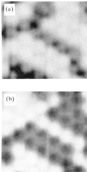
FIG. 3. (a) 100 \times 100\text{-}\text{\AA}^2 tunneling image recorded at tip bias of -1.4\text{ V} , 1\text{ nA} . (b) Simultaneous image of the differential conductivity at the same bias. Bright regions indicate higher differential conductance.
