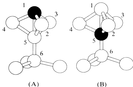
FIG. 4. Two possible locations of the boron atom: (a) T_4 adatom, as other group-III adsorbates; (b) B_5 location, strongly favored. The models are drawn with the relaxed coordinates.
