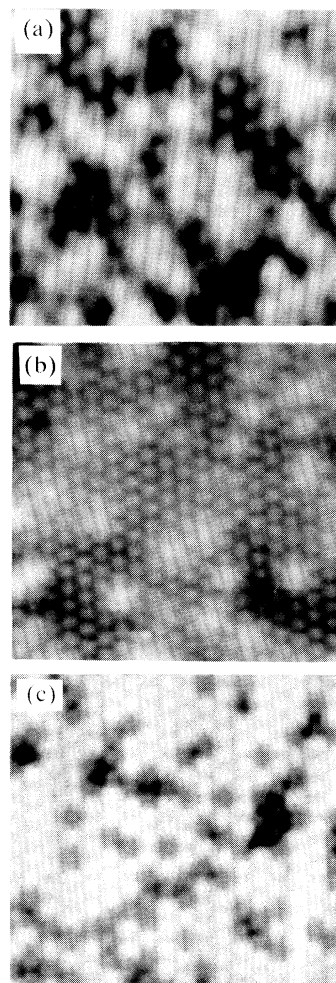
FIG. 1. (a) 100×80-Å 2 tunneling image showing the ( \sqrt{3}\times\sqrt{3} )R30° structure after annealing degenerately boron-doped Si(111) at 1000°C. Tip bias = -1.4 V, 1 nA. (b) 100×100-Å 2 tunneling image of Si(111) prepared by sputtering of B on clean Si(111)7×7. (c) 100×100-Å 2 tunneling image prepared by Si reevaporation on Si(111)( \sqrt{3}\times\sqrt{3} )R30°-B.
