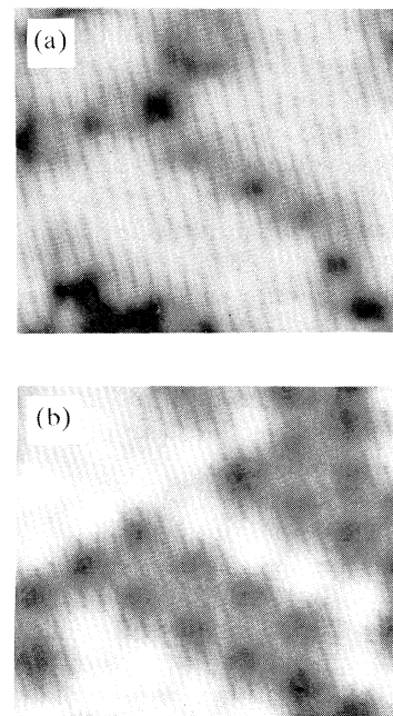
FIG. 3. (a) 100 \times 100\text{-}\text{\AA}^2 tunneling image recorded at tip bias of -1.4\text{ V} , 1\text{ nA} . (b) Simultaneous image of the differential conductivity at the same bias. Bright regions indicate higher differential conductance.
