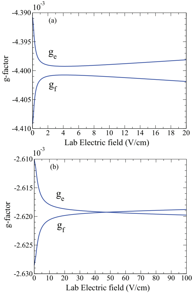
FIG. 2. (Color online) Calculated g_e and g_f for H^3\Delta_1 ^{232}\text{Th}^{16}\text{O} as functions of the electric field. Both Zeeman and Stark interactions with the ^3\Delta_2 and ^3\Pi_{0\pm} states are taken into account. (a) J = 1 and M = 1 . (b) J = 2 and M = 1 .
