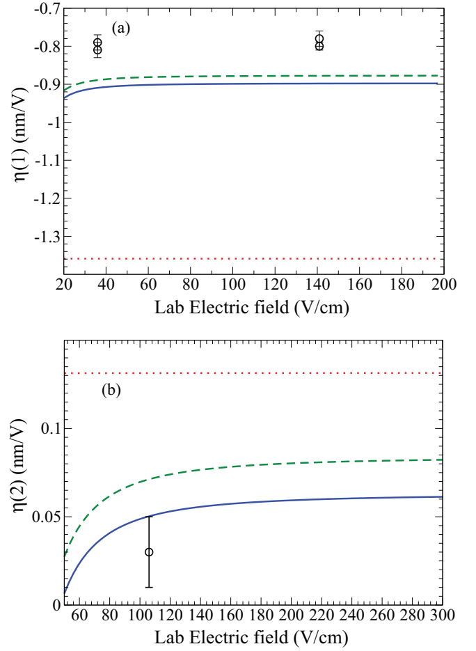
FIG. 3. (Color online) Calculated \eta(J) as functions of the electric field. Solid (blue) curves: Both Zeeman and Stark interactions with the ^3\Delta_2 and ^3\Pi_{0\pm} states are taken into account. Dashed (green) curves: Only the Zeeman interaction with the ^3\Delta_2 and ^3\Pi_{0\pm} states is taken into account. Dotted (red) curves: Both Zeeman and Stark interactions with the ^3\Delta_2 and ^3\Pi_{0\pm} states are omitted. Circles (black): Experimental values. (a) J = 1 and M = 1 . (b) J = 2 and M = 1 .
