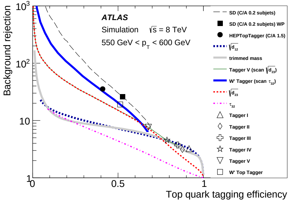
Figure 14: The background rejection as a function of the tagging efficiency of large- R jets, as obtained from MC simulations for 350 \text{ GeV} < p_T < 400 \text{ GeV} and 550 \text{ GeV} < p_T < 600 \text{ GeV} for trimmed anti- k_t R = 1.0 particle-level jets to which the large- R jets are geometrically matched. The HEPTopTagger uses C/A R = 1.5 jets; the other taggers use trimmed anti- k_t R = 1.0 jets. For SD, the cut value of the discriminant \ln \chi is scanned over. Substructure-variable-based taggers are also shown including single scans over the trimmed mass, \sqrt{d_{12}} , \sqrt{d_{23}} , \tau_{32} and scans over cuts on \sqrt{d_{23}} and \tau_{32} for substructure tagger V and the W' top tagger, respectively. The curves are not shown if the background efficiency is higher than the signal efficiency, which for some substructure-variable scans occurs for very low signal efficiencies, i.e. for scans in the tails of the distributions. The statistical uncertainty from the simulation is smaller than the symbols for the different working points and it is no larger than the width of the lines shown.
