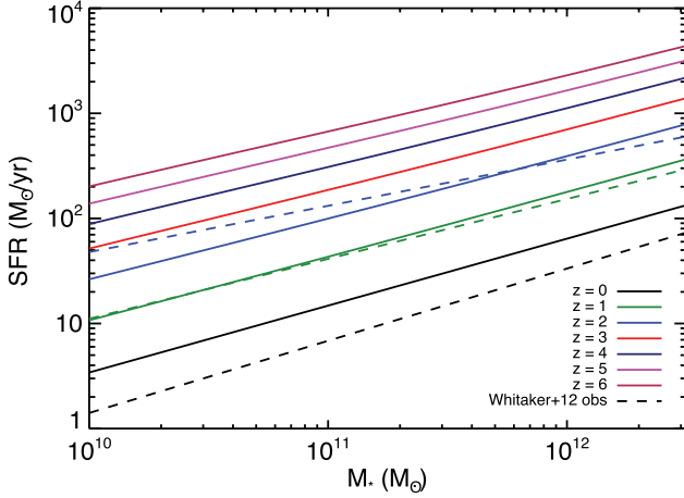
Figure 2. SFR ( M_{\odot} \text{ yr}^{-1} ) versus M_{\star} (M_{\odot}) for model disc galaxies at integer redshifts in the range z = 0-6 (solid lines) and from the observationally derived fitting function of Whitaker et al. (2012) at z = 0, 1 and 2 (dashed lines). The normalization of the relation increases with redshift both because gas fractions are higher and galaxies are more compact. The model agrees reasonably well with the observations except at z \sim 0 , but we shall see that the z \sim 0 contribution to our model SMG population is small. If the SFRs from Whitaker et al. (2012) were used instead of those calculated from equation (10), the z \sim 0 contribution would be even less, so the discrepancy is unimportant.
