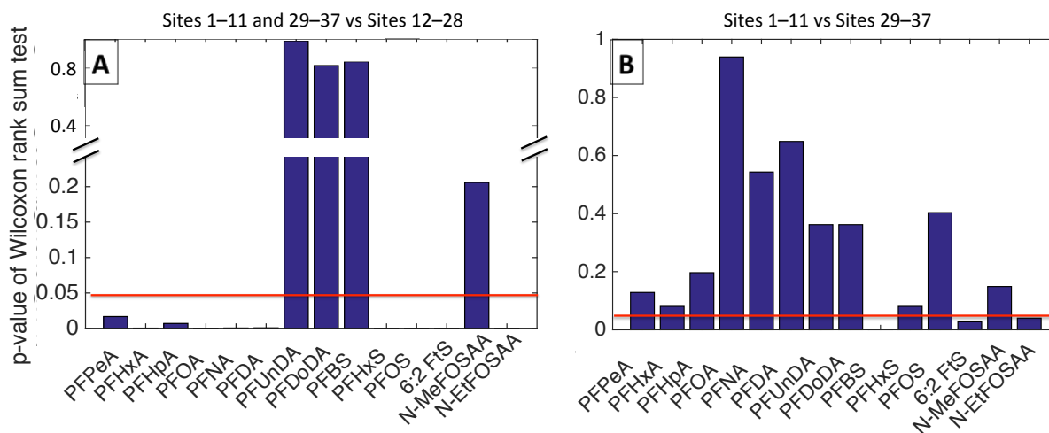
Figure S3. Significance levels for Wilcoxon rank sum tests comparing PFAS concentrations (a) between urban sites (RI sites 1–11 and NY/NJ sites 29–37) and rural sites 12–28 (b) RI sites 1–11 and NY/NJ sites 29–37. Red line denotes p=0.05 , which we use to indicate statistical significance.
