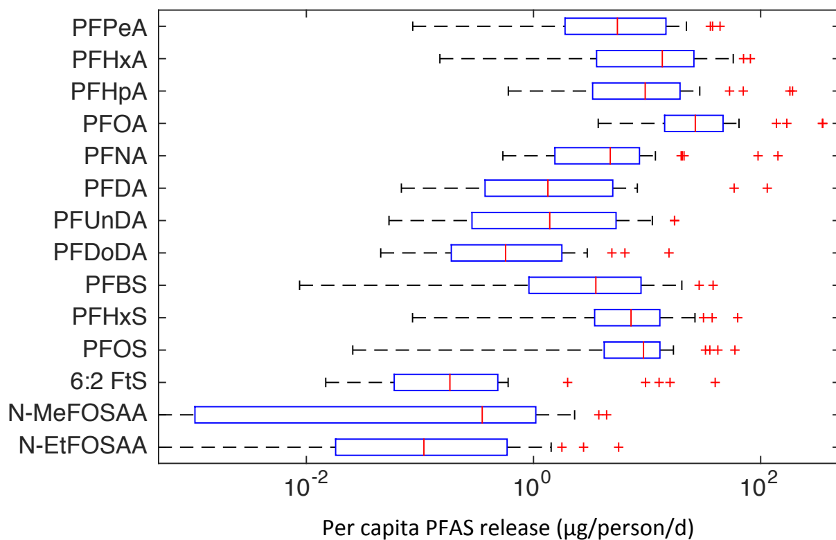
210 Figure S4. Per-capita release of PFAS (µg/person/d) estimated based on measured PFAS 211 concentrations, water flow rate and upstream population at each sampling site.
