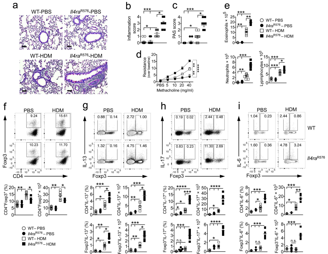
Figure 1. Il4ra R576 polymorphism promotes enhanced lung inflammation and AHR, associated with increased IL-17, IL-6 and IL-13 expression. (a) Representative PAS staining of lung sections isolated from WT and Il4ra R576 mice either sham treated with PBS or immunized and challenged with HDM and analyzed 24 hr after the last challenge (20×, scale bar 50 μm) ( n = 11 counts per field-of-view). (b,c) Inflammation and PAS scores from the group of mice shown in a. (d) Methacholine-induced AHR for the same groups shown in a ( n = 8 mice per group). (e) Absolute numbers of lung tissue eosinophils, neutrophils and lymphocytes, in the respective mouse groups ( n = 5 mice for PBS and 7 mice for HDM groups). (f) Flow cytometric analysis, frequencies and absolute numbers of CD4 + Foxp3 + T reg cells within lung tissue ( n = 8 mice per group). (g-i) Flow cytometric analysis of IL-13 (g), IL-17 (h) and IL-6 (i) expression by CD4 + Foxp3 - T conv or CD4 + Foxp3 + T reg cells within CD90.2 + gated cells (representing all T lymphocytes) in lung tissues of WT and Il4ra R576 mice treated with PBS or HDM ( n = 5 mice for PBS and 7 mice for HDM groups). Results represent means ± s.e.m. from two independent experiments. * P < 0.05 , ** P < 0.01 and *** P < 0.001
