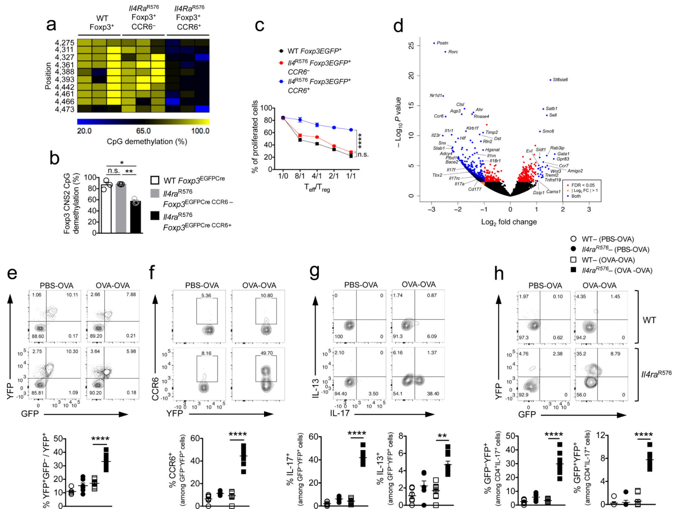
Figure 3. CCR6 + IL-17 + Il4 R576 T reg cells exhibit instability and compromised suppressive activity ( a ) Methylation status of CpG motifs in T reg cells isolated from lung tissue of OVA-sensitized and challenged mice. Numbers on the left side indicate the position of the respective motifs. ( b ) Global methylation status of Foxp3 CNS2 in the respective T reg cell populations ( n = 3 mice per group with 7-12 clones per mouse). ( c ) In vitro suppression of the proliferation of WT responder CD4 + T cells (T eff ) by the respective T reg cell populations ( n = 3 replicates per group) ( d ) Gene expression profiles (volcano plot) of EGFP + CCR6 - versus EGFP + CCR6 + T reg cells isolated by FACS from lung digests of OVA-sensitized and challenged Foxp3 EGFP Il4 R576 mice ( n = 3-4 mice). FDR: false discovery rate; Log 2 FC: Log 2 fold change. ( e ) Flow cytometric analysis and frequencies of exT reg (GFP + YFP + ) cells, plotted as a fraction of exT reg to total T reg cells in lung tissue. ( f,g ) Flow cytometric analysis and frequencies of CCR6 producing ( f ) and IL-17 and IL-13 producing ( g ) exT reg cells in lung tissues. ( h ) Flow cytometric analysis and frequencies of exT reg and T reg cells among CD4 + IL-17 + T conv cells in lung tissues of the respective mouse groups ( n = 6 mice for PBS- and 9 mice for OVA-treated groups for e-h ). Data represent means \pm s.e.m. from two independent experiments. * P < 0.05 , ** P < 0.005 and **** P < 0.0001 by one-way ANOVA
