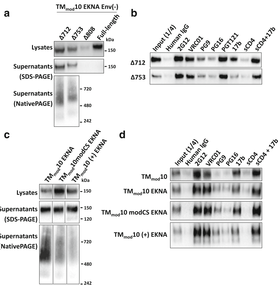
Fig. 3 Effects of cytoplasmic tail and cleavage site modifications on TM_{mod}10 Env. a The TM_{mod}10 EKNA variant has the E168K + N188A changes that allow the HIV-1 JR-FL Env to be recognized by the PG9 and PG16 antibodies [96–99]. The full-length TM_{mod}10 EKNA Env or the TM_{mod}10 EKNA variants with a deleted ( \Delta 712 ) or truncated ( \Delta 753 and \Delta 808 ) cytoplasmic tail were expressed in 293T cells. The cell lysates and supernatants were analyzed by SDS-PAGE, and the cell supernatants by Blue Native PAGE. The gels shown in this figure were Western blotted with a polyclonal goat anti-gp120 antibody. Addition of the cytoplasmic tail did not prevent TM_{mod}10 EKNA expression in cells, but only the TM_{mod}10\Delta 753 EKNA glycoprotein with the shortest tail was secreted. The secreted TM_{mod}10\Delta 753 Env was mainly dimeric based on the Blue Native gel. b The TM_{mod}\Delta 712 and TM_{mod}\Delta 753 EKNA Envs precipitated from the supernatants of expressing cells by the indicated antibodies are shown. The antigenic profiles of these two Envs are similar. c TM_{mod}10 EKNA variants with modifications of the cleavage site, including a wild-type cleavage site (+) or a flexible linker ((GGG) 4 ) replacing the cleavage site (modCS), were analyzed as in a . Note that the TM_{mod}10 (+) EKNA Env is partially cleaved, as indicated by the presence of a gp120 band on SDS-PAGE. d Precipitation of the TM_{mod}10 and TM_{mod}10 EKNA variants by the indicated antibodies is shown. Data are representative of those obtained in at least two independent experiments
