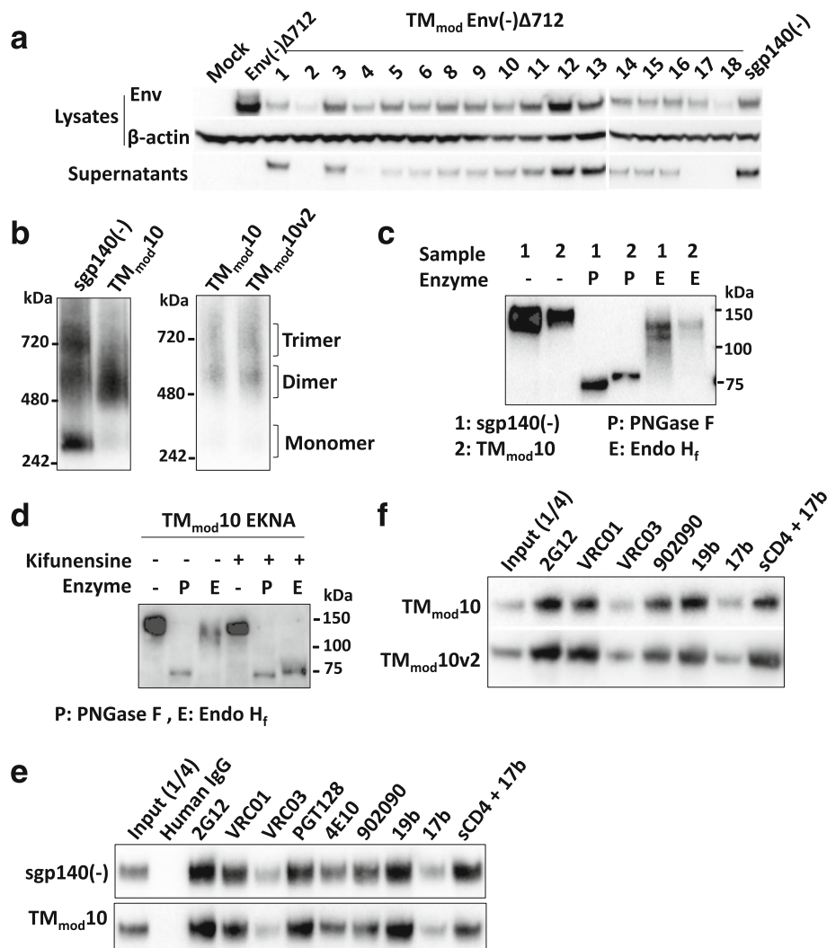
Fig. 2 Characterization of TM mod mutant Envs. a Cellular lysates and supernatants from 293T cells that were mock-transfected or transfected with TM mod Env DNAs were Western blotted. Western blots shown in this figure used goat anti-gp120 antibody or a mouse anti-β-actin control. The TM mod Envs with at least two new charged residues in the transmembrane region were secreted. The control TM mod 18 Env was inefficiently expressed and not secreted. The sgp140(-) Env lacks the transmembrane region. b The secreted Envs were analyzed by Blue Native PAGE. The sgp140(-) glycoprotein migrated as a heterogeneous mixture of monomers, dimers and trimers. The representative TM mod 10 protein migrated predominantly as a dimer. The TM mod 10v2 glycoprotein was also largely dimeric. Note that HIV-1 Envs migrate more slowly than expected in Blue Native gels. c Transfected cell supernatants containing sgp140(-) and TM mod 10 Envs were either mock-treated or treated with PNGase F (which removes all N-linked glycans) or Endo H f (which removes only high-mannose glycans). The Western blot shows that both sgp140(-) and TM mod 10 Envs resist Endo H f treatment, which indicates that they contain mostly complex carbohydrates. d Transfected cells expressing the E168K + N188A (EKNA) variant of TM mod 10, which allows HIV-1 JR-FL Envs to be recognized by the PG9 and PG16 neutralizing antibodies [96–99], were incubated with 50 mM kifunensine (a mannosidase I inhibitor). Cell supernatants were collected, deglycosylated with PNGase F or Endo H f , and Western blotted. Addition of kifunensine converted TM mod 10 glycosylation from mostly complex glycans to high-mannose glycans. e, f Cell supernatants containing the indicated soluble glycoproteins were precipitated with the indicated antibodies, and the precipitates were Western blotted with goat anti-gp120 antibody. The three soluble Envs exhibit a similar pattern of antigenicity. One-fourth volume of the supernatant used for immunoprecipitation was analyzed in the input lane. Data are representative of those obtained in at least two independent experiments
