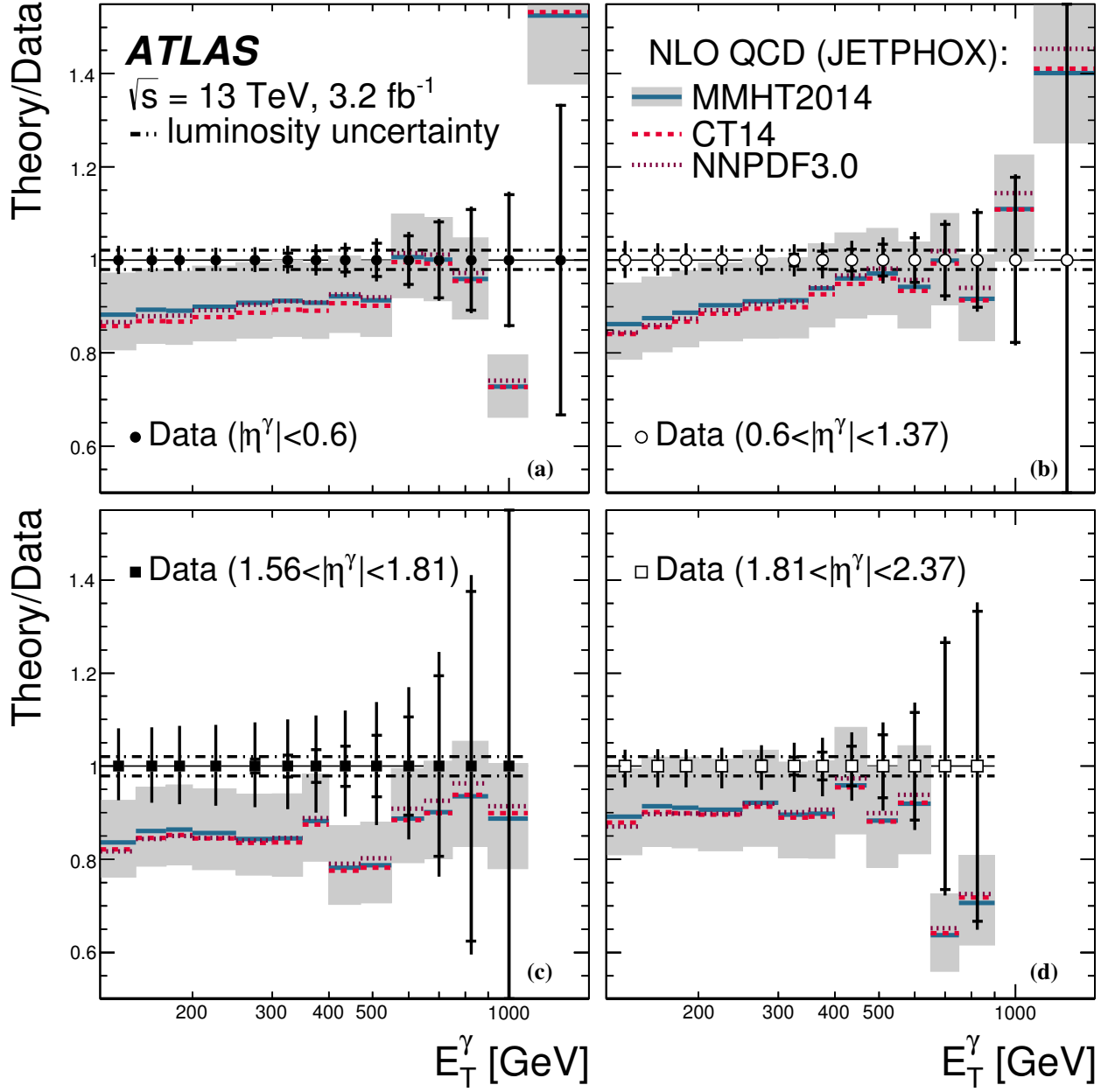
Figure 3: Ratio of the NLO pQCD predictions from JETPHOX based on the MMHT2014 PDFs to the measured cross sections for isolated-photon production (solid lines) as a function of E_T^\gamma in (a) |\eta^\gamma| < 0.6 , (b) 0.6 < |\eta^\gamma| < 1.37 , (c) 1.56 < |\eta^\gamma| < 1.81 and (d) 1.81 < |\eta^\gamma| < 2.37 . The inner (outer) error bars represent the statistical uncertainties (statistical and systematic uncertainties, excluding that on the luminosity, added in quadrature), the dot-dot-dashed lines represent the uncertainty due to the luminosity measurement and the shaded bands display the theoretical uncertainty of the calculation based on the MMHT2014 PDFs. The ratio of the NLO pQCD predictions based on the CT14 (dashed lines) or NNPDF3.0 (dotted lines) PDF sets to the data are also included.
