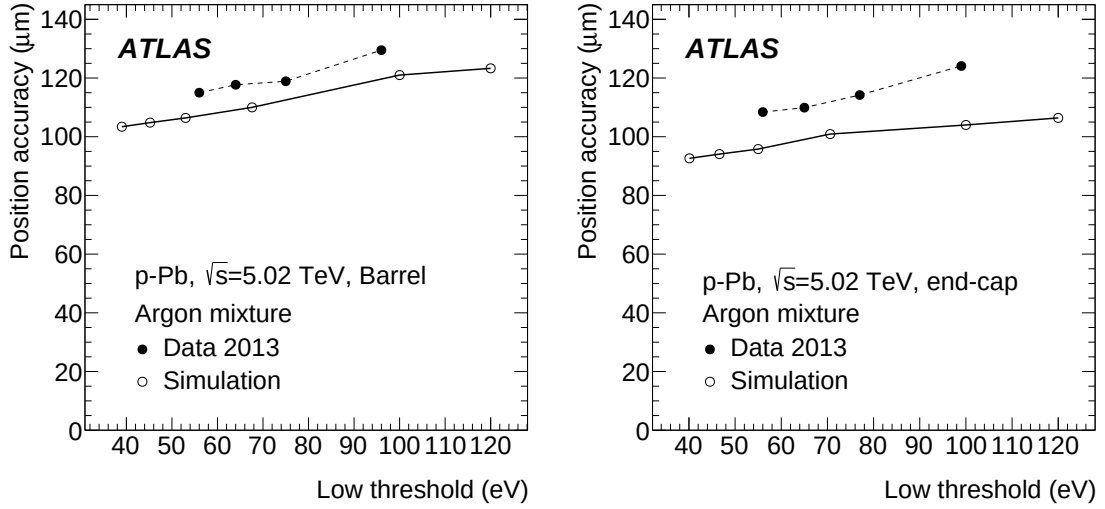
Figure 16: Straw track position measurement accuracy as a function of the threshold setting for the barrel modules (left) and end-cap wheels (right) filled with an Ar-based gas mixture, for the data (solid circles) and simulation (open circles).
