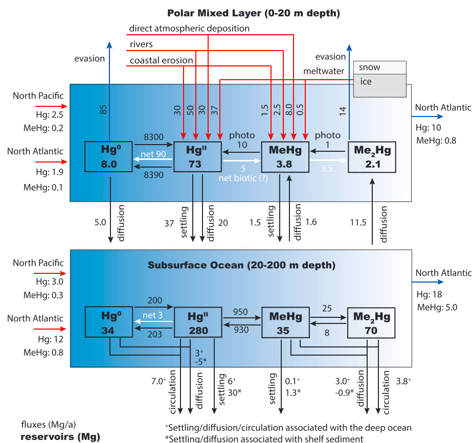
Figure 5. Reservoirs (Mg) and mass flows ( \text{Mg a}^{-1} ) in the Arctic polar mixed layer (PML) and subsurface ocean. Red arrows indicate external sources, blue arrows denote losses out of the system, black arrows show internal fluxes, and white arrows indicate net fluxes. Figure 3 shows fluxes for the deep ocean, which cannot be resolved on species-specific basis due to lack of data.
