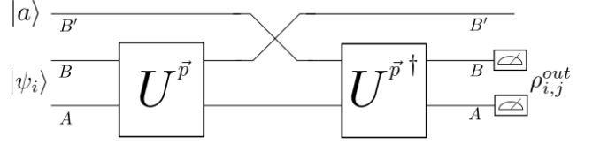
Figure 2. A quantum autoencoder circuit. The goal is to find \vec{p} such that the averaged F(|\psi\rangle_i, \rho_{i,\vec{p}}^{out}) is maximized.
