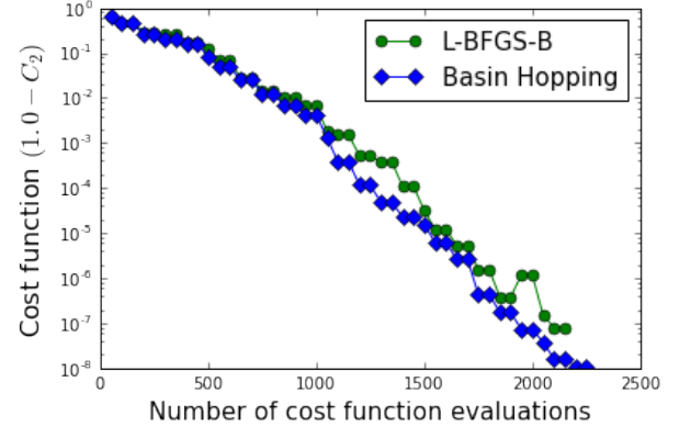
Figure 7. A plot of the cost function versus the number of cost function evaluations during the training process. This example corresponds to a quantum autoencoder for compression of wavefunction of H_2 from 4 to 2 qubits using circuit A with a training set of six ground states. We compared the L-BFGS-B and the Basin-Hopping algorithms for optimization.
