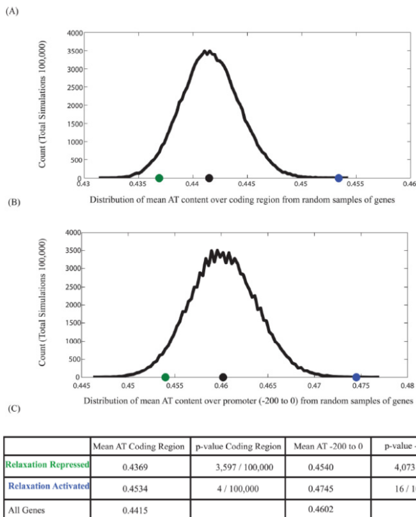
Figure S2.7: Statistical significance of increased and decreased AT content in monotonically relaxation activated and monotonically relaxation repressed genes, respectively.
