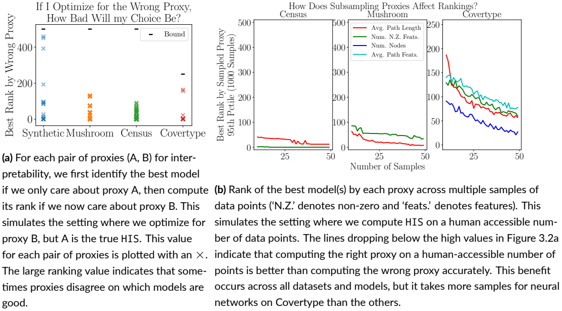
Figure 3.2: Determining interpretability on a few points is better than using the wrong proxy.
