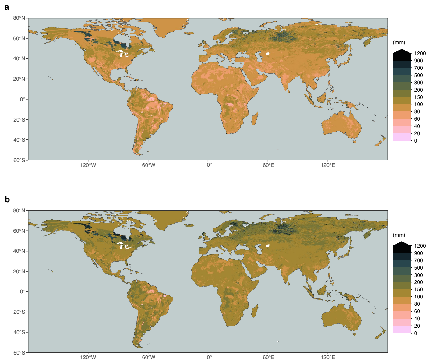
Extended Data Fig. 5 | Integrated soil water holding capacity in the soil. Integrated soil water holding capacity across the top 1 m (a) and the top 2 m (b). Values are calculated based on soil texture information from a gridded version 30 of the Harmonized World Soil Database 29 and pedo-transfer functions based on
