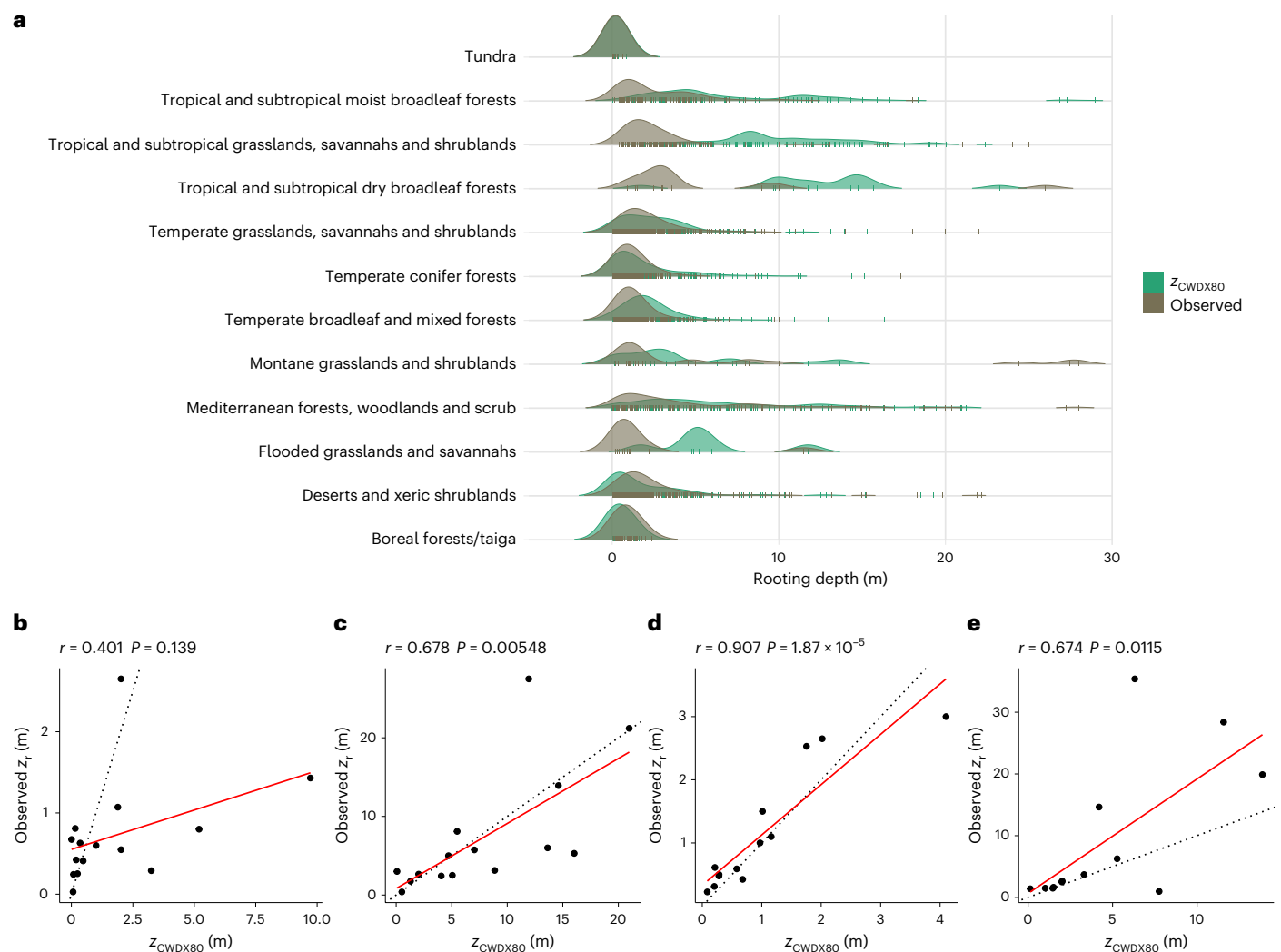
Fig. 4 | Modelled and observed rooting depth by biome. a , Kernel density estimates of observed and predicted ( z_{CWDx80} ) rooting depth by biome, based on data aggregated by sites, shown by vertical coloured tick marks. b–e , The 10% ( b,d ) and 90% ( c,e ) quantiles of observed versus predicted ( z_{CWDx80} ) rooting depth by biome of all data ( b,c ) and of a subset of the data where the WTD was
