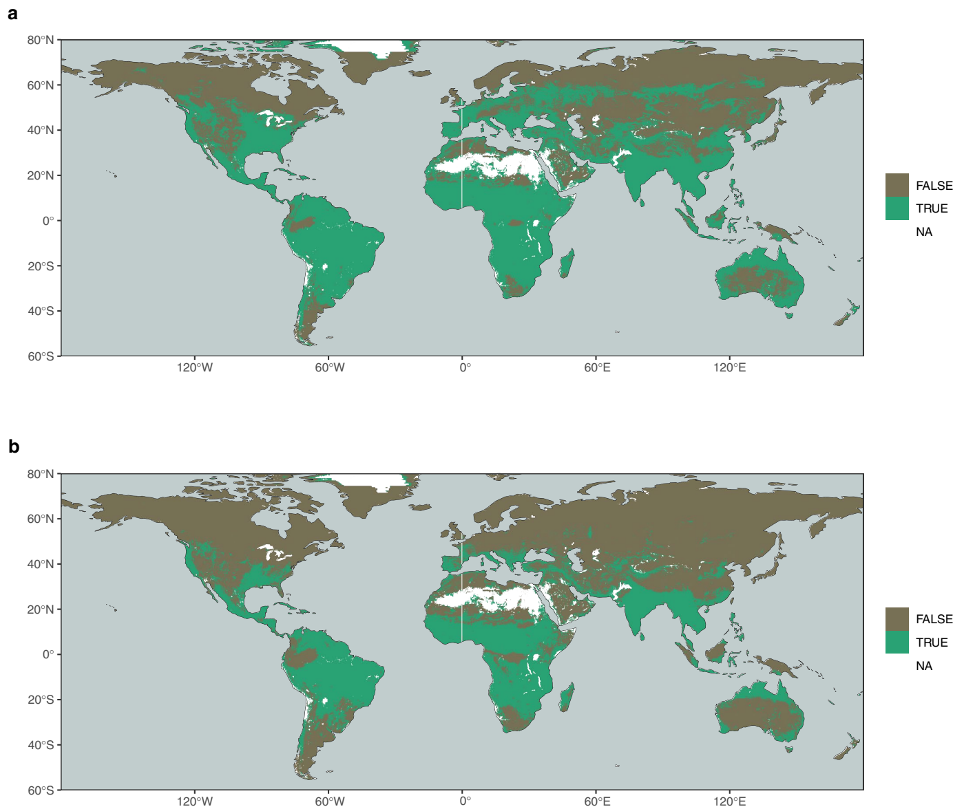
Extended Data Fig. 6 | Locations of plant access to deep water storage. Plant access to deep water storage. Green colors indicate regions where S_{\text{CWDx80}} suggests a rooting zone water storage capacity larger than the integrated water holding capacity across the top 1 m (a) and 2 m (b).
