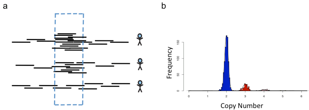
Figure 3.5. Genome STRiP copy number genotyping utilizes WGS read depth.
