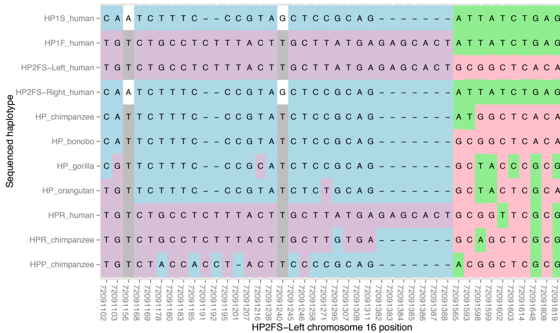
Supplementary Figure 1. HP contains paralogous gene conversion from HPR and a highly diverged region. An alignment of the structurally variant region for human structural haplotypes and other primates shows distinct polymorphic sections. The paralog which provided the sequence is indicated, excluding the Marmoset and Squirrel Monkey sequences as these primates lack the triplication. Only the fixed differences between human HP structural forms are plotted. The blue and lavender region shows that human HP1F and HP2FS-Left have 33 derived mutations (with respect to the chimpanzee and bonobo HP ) which match the human HPR gene. The series of mutation that gave rise to the highly diverged region is unclear, as the great apes are also highly polymorphic in this region, and multiple bases have potentially deep coalescence.
