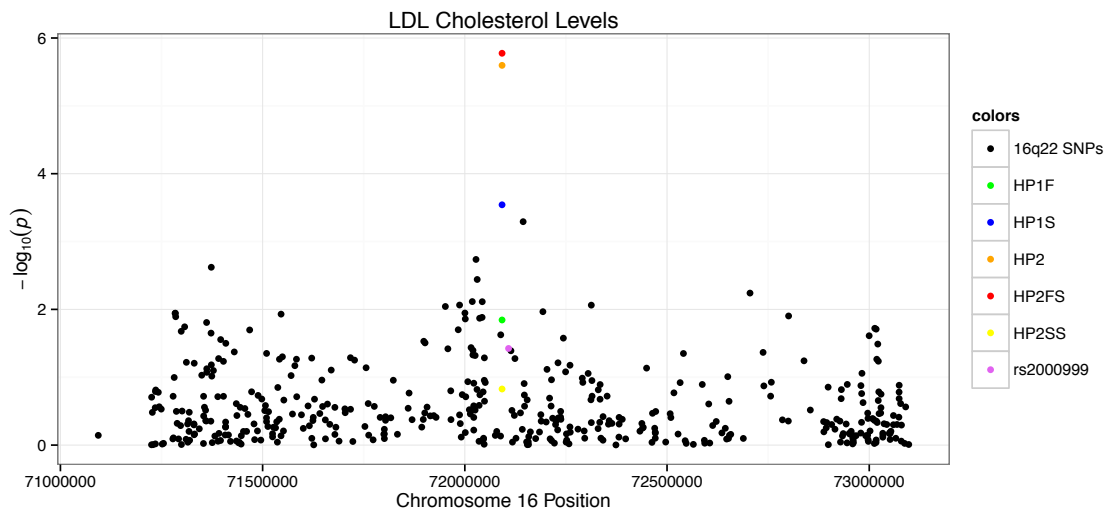
Figure 5.3. HP2 associates to total and LDL cholesterol levels. Regional SNPs are shown in black, while the GWAS index SNP (rs2000999) is shown in pink. Other colors indicate HP structures (see legend). (a) HP2 is most highly associated to total cholesterol levels. (b) HP2FS is the structural haplotype most associated with LDL cholesterol levels.
