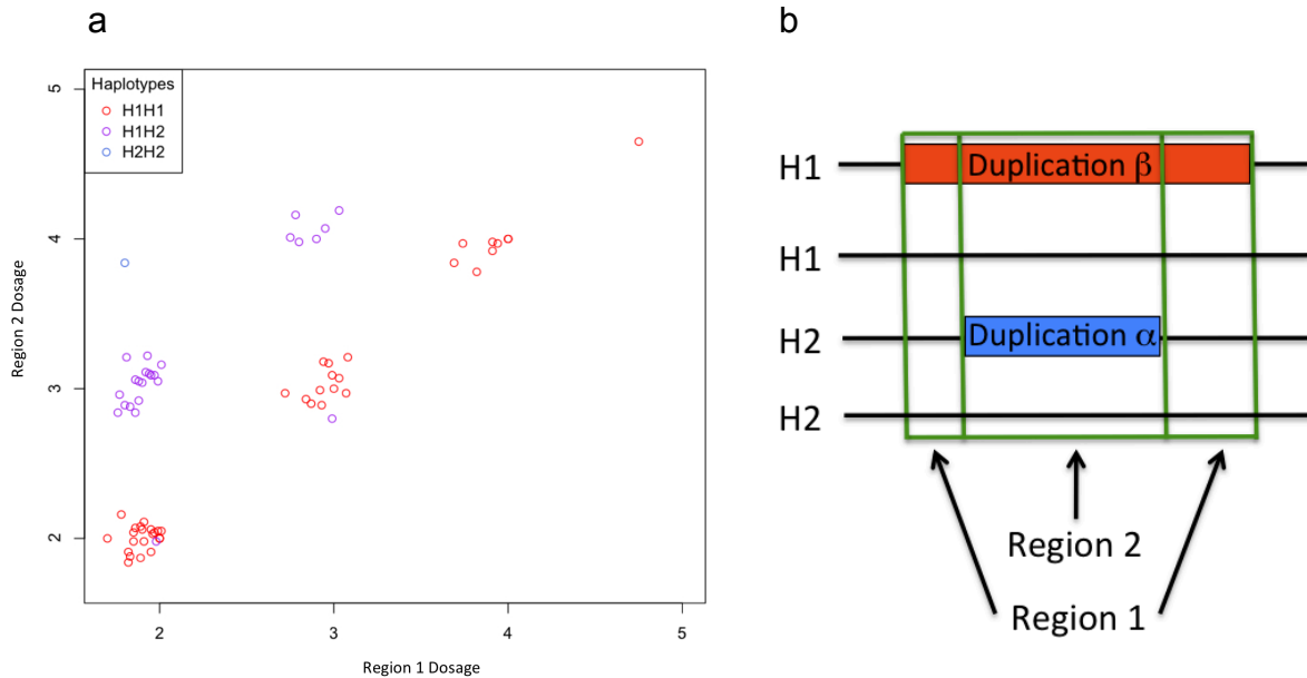
Figure 3.7. Relating the inversion to duplications. Comparison of copy number in Region 1 and Region 2 in the context of H1/H2 haplotype orientation makes it clear that copy number is influenced by two separate duplication polymorphisms segregating with different inversion states. Three main observations underlie this determination. (1) Copy number of Region 1 was always equal to copy number of Region 2 in H1 homozygotes. (2) Copy number in Region 2 was (in all but two cases, described below) equal to the sum of (i) copy number of Region 1 and (ii) the number of H2 haplotypes that an individual carries. This indicated that a duplication of Region 2 is present on most H2 haplotypes. (3) Copy number in Region 1 was only greater than two in individuals with at least one H1. These data indicated the existence of a long duplication which overlaps Region 1 and Region 2 segregating on the H1 background, and a shorter duplication overlapping Region 2 segregating on the H2 background.
