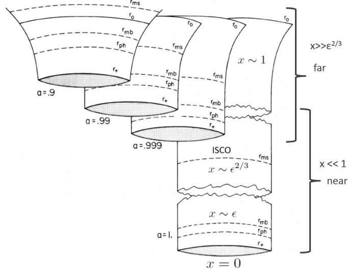
Figure 3.2: The well-known diagram of [81] overlaid with corresponding regions of the dimensionless coordinate x that we consider. The dashed lines illustrate the BL radii of the ISCO r_{\text{ms}} , the marginally bound orbit r_{\text{mb}} , and the photon orbit r_{\text{ph}} . Also shown are the horizon r_+ and a constant ( \epsilon -independent) BL radius r_0 . (Note that we use the notation x_0 for the ISCO radius in the main body.) The “cracks” in the throat illustrate infinite proper radial distance on a BL slice in the extremal limit. They can also be interpreted as signaling the presence of three physically distinct extremal limits (App. A).
