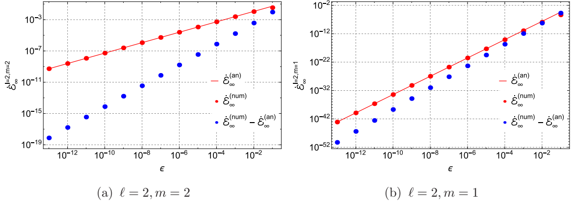
Figure 3.3: Energy flux to infinity for the 2-2 and 2-1 modes in the gravitational case. The analytic results and numerical results are denoted by \dot{\mathcal{E}}_\infty^{(\text{an})} and \dot{\mathcal{E}}_\infty^{(\text{num})} , respectively. The 2-2 mode has h \simeq 1/2 + 2.050928i and hence an exponent of p = 2/3 , while the 2-1 mode has h \simeq 2.419070 and an exponent of p \simeq 3.225427 . The 2-2 mode also has oscillations, too small to be seen on this scale but clearly visible in Fig. 3.4. Note that the results in this figure have been adimensionalized so that \dot{\mathcal{E}}^{(\text{here})} \equiv (M/m_0)^2 \dot{\mathcal{E}} .
