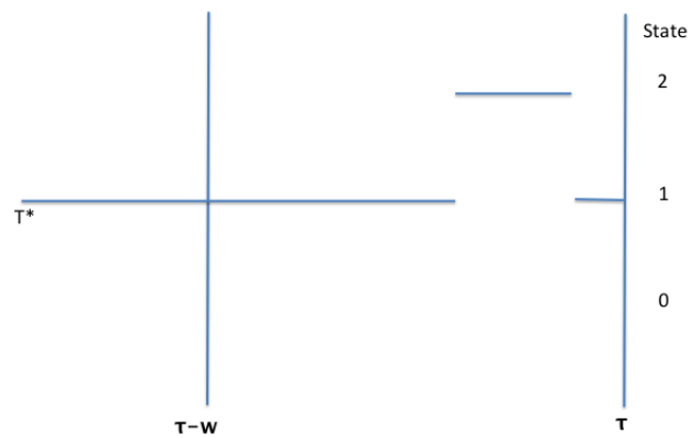
Figure 2.2: Two different duration data (a) and (b) have identical sample path (1 \rightarrow 2 \rightarrow 1) as shown in (c)
