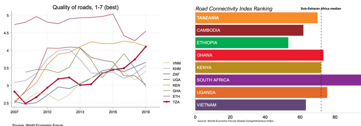
Figure 44: Road infrastructure
