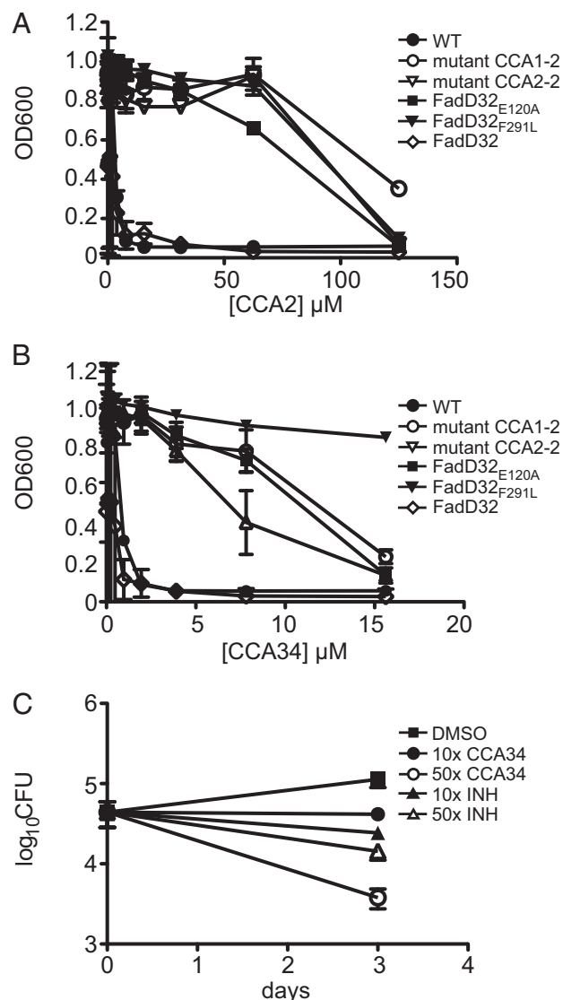
Fig. 2. Activity of substituted coumarins in vitro and in macrophages. Mutants selected on substituted coumarin inhibitors and WT M. tuberculosis expressing mutant Fadd32 epismally are resistant to high concentrations of (A) CCA2 and (B) CCA34. (C) Substituted coumarin inhibitors are effective at treating infected human PBMC derived macrophages. For the macrophage infection experiment, macrophages were infected at MOI = 1 and were carried out for 3 d. All treatments relative to DMSO control gave P < 0.02 ( n = 3 ) by the Mann-Whitney U test. All experiments were repeated a minimum of three times, and a representative experiment is shown. Error bars are SD.
