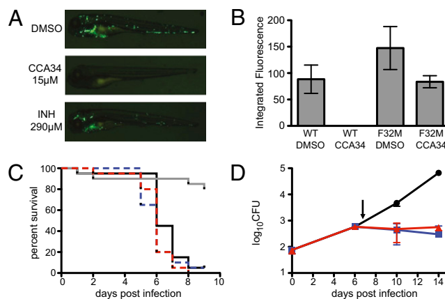
Fig. 4. Validation of FadD32 as a targetable and essential protein for in vivo infection. (A) CCA34 prevents replication of M. marinum in zebrafish. Treatment of infected zebrafish with 15 \mu M CCA34 inhibits bacterial proliferation. (B) Mutation of FadD32 confers resistance to CCA34 in vivo. Fish were infected with WT or FadD32 mutant (F32M) M. marinum , and day 3 bacterial loads were quantified from fluorescent images ( n = 5 for each condition). (C) Treatment of infected zebrafish with CCA34 prolongs survival for embryos infected with WT but not F32M. Solid black line, WT/DMSO; solid gray line, WT/15 \mu M CCA34; dashed red line, F32M/DMSO; dashed blue line, F32M/15 \mu M CCA34. For all conditions vs. WT infected DMSO treated fish, P < 0.0001 by the log rank test ( n = 20 ). For all zebrafish figures a representative experiment of three is shown. (D) Efficacy of CCA34 in a mouse model of tuberculosis. BALB/C mice infected with M. tuberculosis via aerosol were treated with INH (25 mg/kg) or CCA34 (35 mg/kg) beginning on day 7 after infection (indicated by the black arrow) for a total of 7 d. Error bars are SD. *P < 0.02 ( n = 5 ) using the Mann-Whitney U test. A representative experiment of two is shown.
