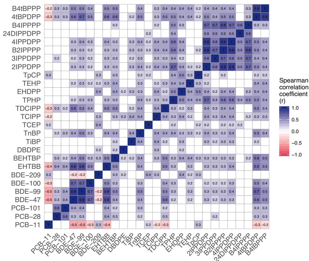
Figure 2.5. Significant ( p<0.028 ) Spearman correlation coefficients for chemicals detected in at least one-third of silicone wristband samples within a country ( n=130 ).
