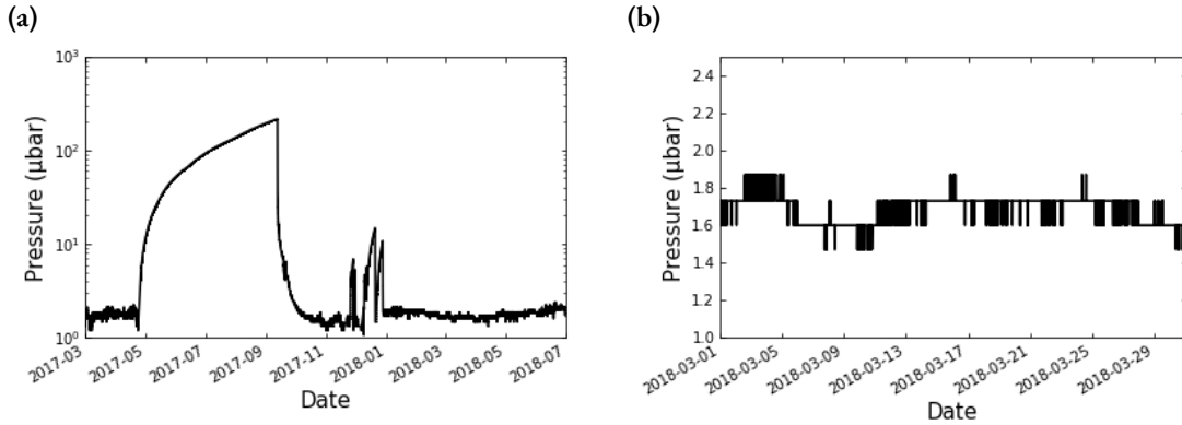
Figure 2.3: Spectrograph pressure inside the KiwiSpec spectrograph. The plotted measures were taken between 2017 March and 2018 July. A power outage at the MINERVA facility resulted in the pressure spike seen during 2017 mid-April. Alongside is plotted the month of 2018 March to show the shorter term stability after this was resolved. Note the pressure shown here is quantized because we are approaching the limit of our Granville Phillips 275 Convectron Gauge.
