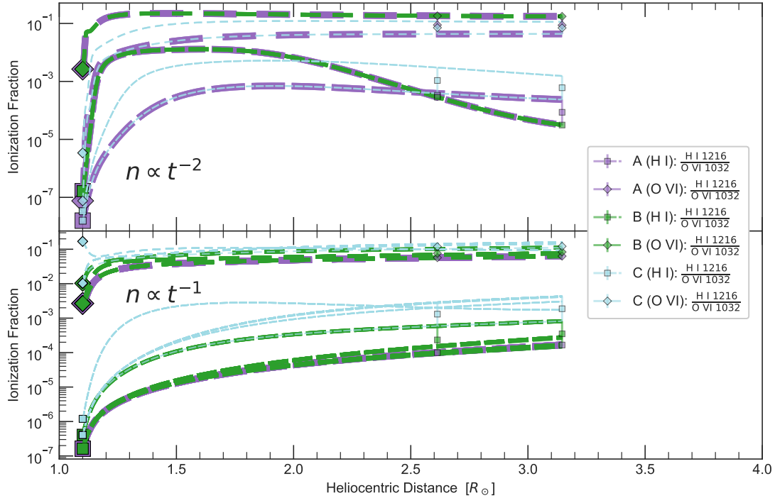
Figure 3.9: Resultant set of ionization fraction profiles after using the Q_{AHH} heating function and constraints from only the \frac{\text{H I } 1216}{\text{O VI } 1032} ratio.
