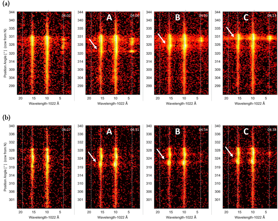
Figure 3.4: For four exposures, the UVCS panel showing the O VI doublet lines is presented. (a) This row corresponds to the last four exposures with the slit at d_H = 2.6 R_\odot . (b) This row corresponds to the last four exposures with the slit at d_H = 3.1 R_\odot .
