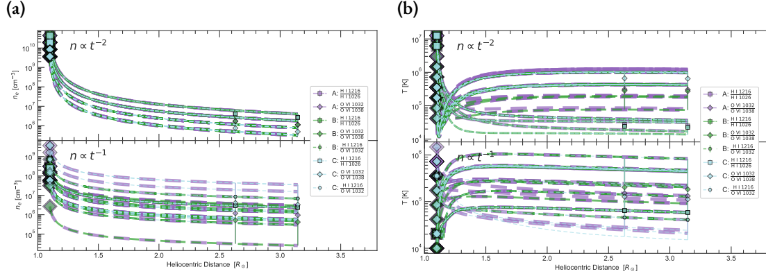
Figure 3.8: Resultant set of electron density and temperature profiles after using the Q_{KR} heating function where \alpha_B = 2 . The square, diamond, and hexagon symbols located at 2.6 and 3.1 R_\odot are arbitrarily positioned in the middle of their respective upper and lower limits for visual clarity. The vertical position of this symbol is not statistically more significant than other values within its range. (a) These model densities have corresponding temperatures, velocities, and ionization states that yield an intensity ratio congruent to the data. (b) These model temperatures have corresponding densities, velocities, and ionization states that yield an intensity ratio congruent to the data.
