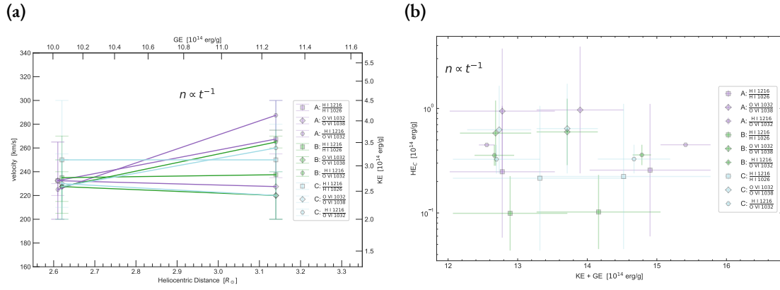
Figure 3.14: Observationally constrained models using the Q_n^2 heating parameterization.
