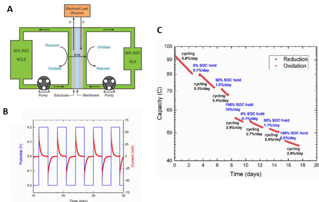
Figure 7. (a) Schematic of unbalanced, compositionally-symmetric flow cell. (b) Example of symmetric cell potentiostatic cycling protocol. (c) Semi-log plot of unbalanced, compositionally-symmetric cell cycling of 50% SOC 0.1 M DHAQ in 1 M KOH with cycling pauses at different SOC. Temporal capacity fade rates from slopes of each cycling segment are denoted in black text. Capacity loss and SOC of CLS during 24-hour pauses are denoted in blue text. Reprinted with permission from ref 33. Copyright 2018 Electrochemical Society.
