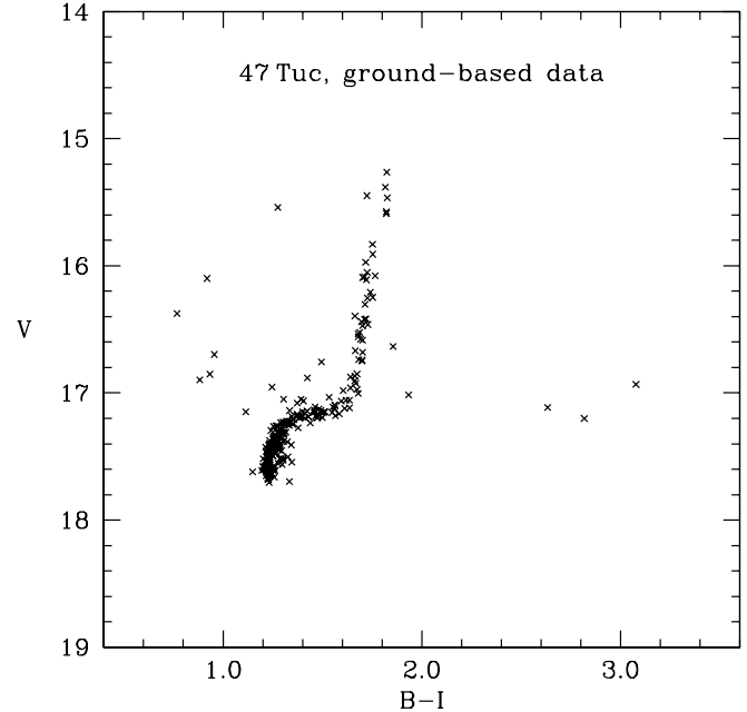
Fig. 4.—Hertzprung-Russell diagram of 250 stars observed from the ground in the cluster 47 Tuc and used to define a photometric transformation between ACS passbands and the Johnson/Cousins system as calibrated by Landolt (1992). These stars were hand selected as those that are well detected in both the ACS images and ground-based images from Stetson (2000). Each of the ground-based points is based on 25–37 independent measurements, with a final photometric uncertainty of 2–3 millimag.
