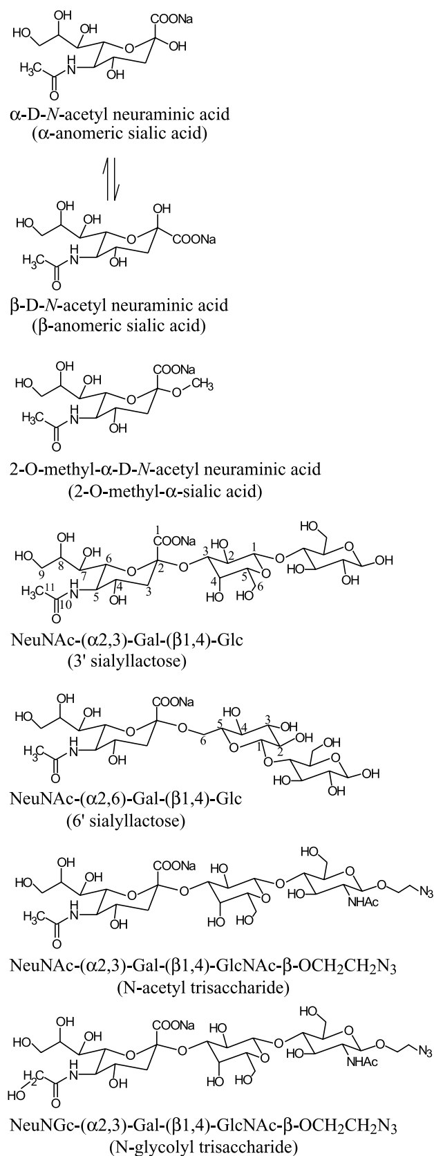
FIG. 1. Structures of the sialosides used in the binding analysis. A short form of the name for each compound is given in parentheses below the complete name. The numbering scheme for the carbons of
