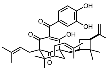
eugeniaphenone (25)
