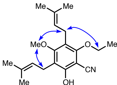
Key 1D nOe correlations.
