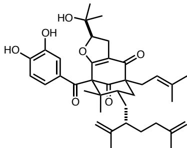
garcinialiptone C (54)
