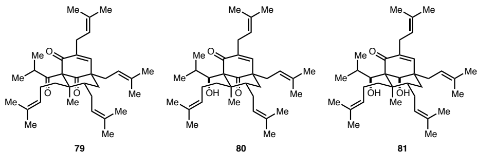
Figure 1.13. Semisynthetic hyperforin derivatives lacking C4 functionality.
