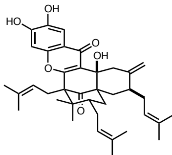
symphonone I (253)
