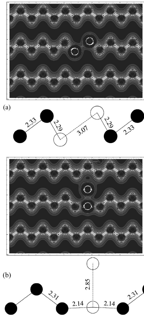
FIG. 3. Same as in Fig. 2 for the configurations: (a) S_{25} and (b) S_{21-v} .
