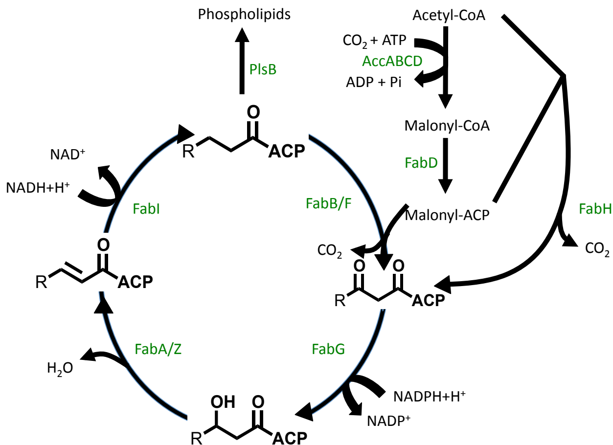
Figure 1.2. Overview of fatty acid synthesis in E. coli . See text for details.
