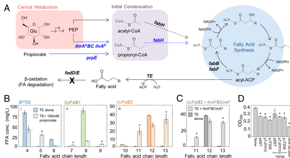
Figure 2.2. Engineering production of all even- and odd-length Medium-Chain Fatty Acids (MCFAs) in E. coli . (A) The ketoacyl synthase (KAS) FabH elongates acetyl-CoA to form a four-carbon β-ketoacyl ACP, which is reduced to C4 acyl-ACP. In subsequent rounds of fatty acid synthesis, the KAS's FabB and FabF elongate acyl-ACPs 2 carbons at a time to yield a range of even-chain-length fatty acyl-ACPs. Incorporation of propionyl-CoA in place of acetyl-CoA causes production of odd-chain acyl-ACPs; propionyl-CoA can be produced from propionate ( prpE ) or from expression of a genetic cassette that increases flux through the isoleucine pathway ( thrA fr BCilvA fr ) [15]. Acyl-ACPs can be hydrolyzed to free fatty acids (FFAs) by an appropriate thioesterase (TE). Fatty acid degradation can be blocked by knocking
