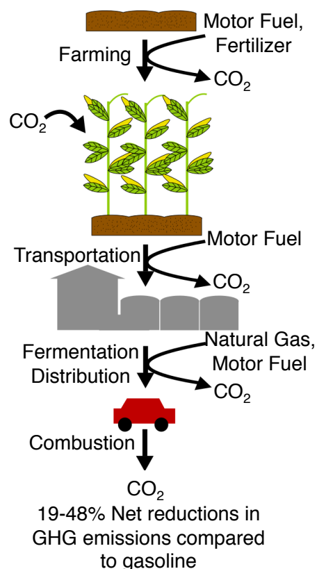
Figure 1.1. Potential for gasoline and ethanol replacement with advanced biofuels. A) United States GHG emissions by economic sector (Data from [2] and [3]). B) Ethanol production process with GHG sources and sinks indicated (Data from [6]).
