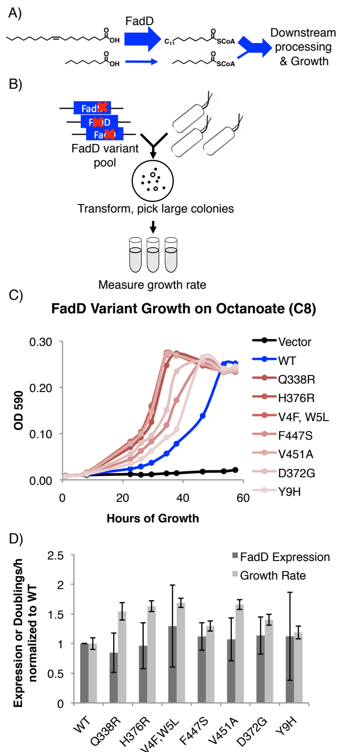
Figure 4.1. FadD mutants generated by error prone PCR increase E. coli \Delta fadR growth rate on octanoate without increasing FadD expression. A) FadD catalyzes the first step in E. coli growth on fatty acids but has low activity on fatty acids shorter than 10 carbons. B) Error prone PCR and FadD screening scheme (Materials and Methods). C) Growth of E. coli \Delta fadR expressing the indicated C-terminally His 6 -tagged FadD mutants generated by error prone PCR from vector
