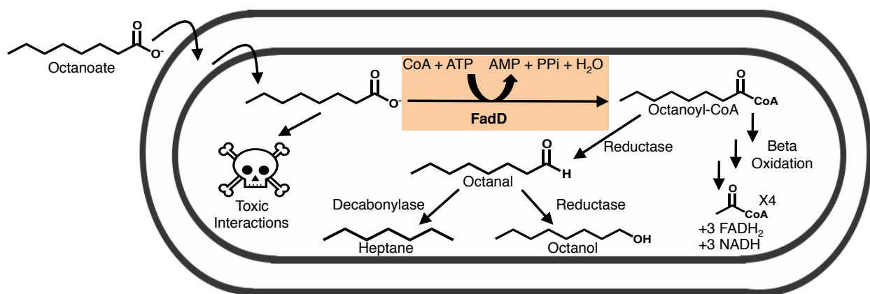
Figure 3.1. Potential pathways for octanoate catabolism and commodity production in E.coli . Octanoate can cross the E.coli outer and inner membranes by simple diffusion [12] and causes cellular toxicity through poorly understood mechanisms [14-16], but may also be catabolized through \beta -oxidation starting with its conversion into octanoyl-CoA by the long chain fatty acyl-CoA synthetase, FadD (highlighted in orange). After this activation step, octanoyl-CoA may be iteratively degraded to acetyl-CoA with the concomitant production of reducing equivalents by other enzymes in \beta -oxidation. Fatty acyl-CoAs can be converted into aldehydes by acyl-CoA reductases [1-3,5,19] and there are likely reductases that can convert octanoyl-CoA into octanal which could later be further decarbonylated or reduced into heptane or octanol respectively [4,5].
