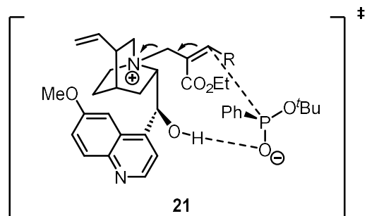
Figure 1.7 Kinetic resolution of secondary phosphine oxides via enantioselective quinine-catalyzed reaction with allylic carbonates.
