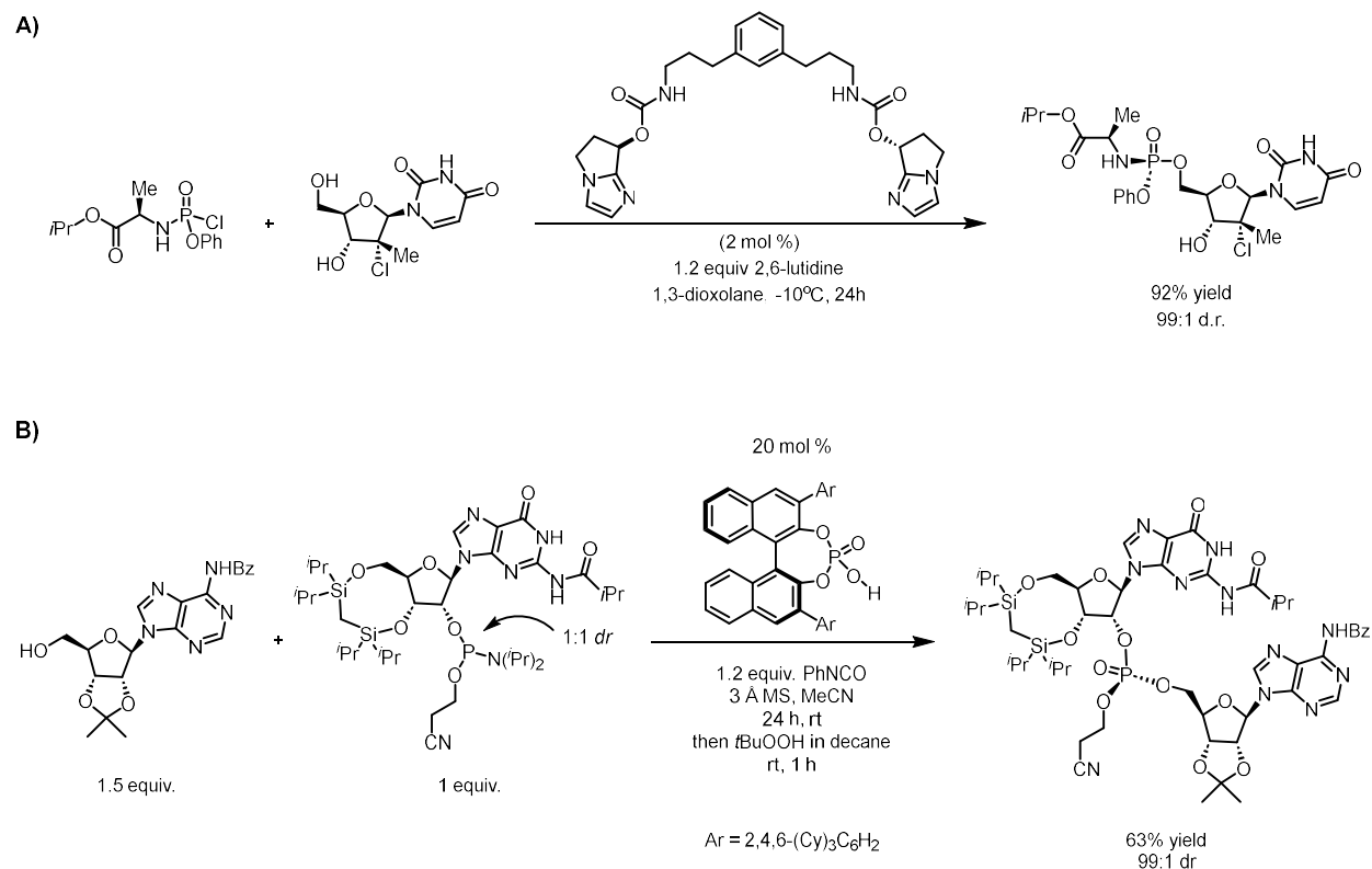
Figure 2.3 Synthetic approaches to stereogenic-at-P(V) targets using stereoselective catalysis.
