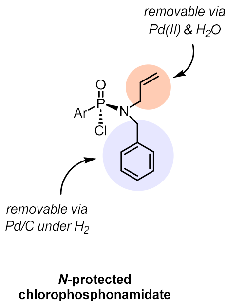
Figure 2.15 N -protected chlorophosphonamidate building block.
