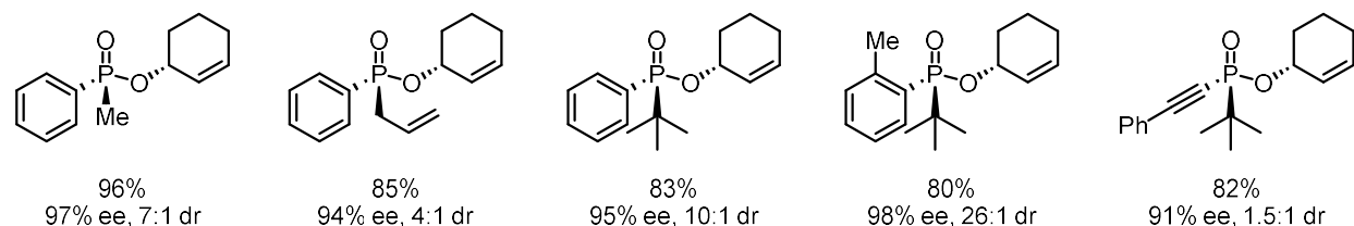
Figure 3.1 Asymmetric synthesis of phosphinate esters via Pd-catalyzed allylic alkylation of phosphinic acids.
