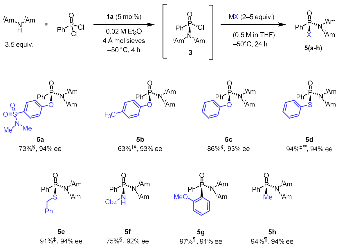
Figure 2.8 Scope of nucleophiles for enantiospecific substitution with 3 . Reactions were carried out on 0.2 mmol scale. Yield values correspond to chromatographically purified, isolated products. The absolute stereochemistry of the products was assigned based on the x-ray crystal structure of 10 . ‡Reaction was carried out using two-pot procedure involving isolation of 3 and subsequent reaction with 2 equivalents of nucleophile. §Reaction was carried out using one-pot procedure without isolation of 3 with 5 equivalents of nucleophile. ¶Reaction was carried out using two-pot procedure involving isolation of 3 and subsequent reaction with 5 equivalents of nucleophile. #Reaction was carried out on 0.9 mmol scale. **Reaction was carried out on 1.0 mmol scale.
