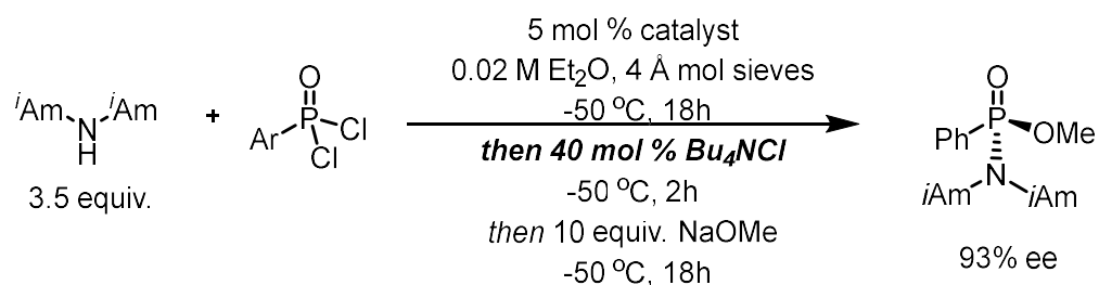
Scheme S2.1 Enantioenriched chlorophosphonamidate 3 formed under reaction conditions does not undergo racemization in the presence of \text{Bu}_4\text{NCl} .
