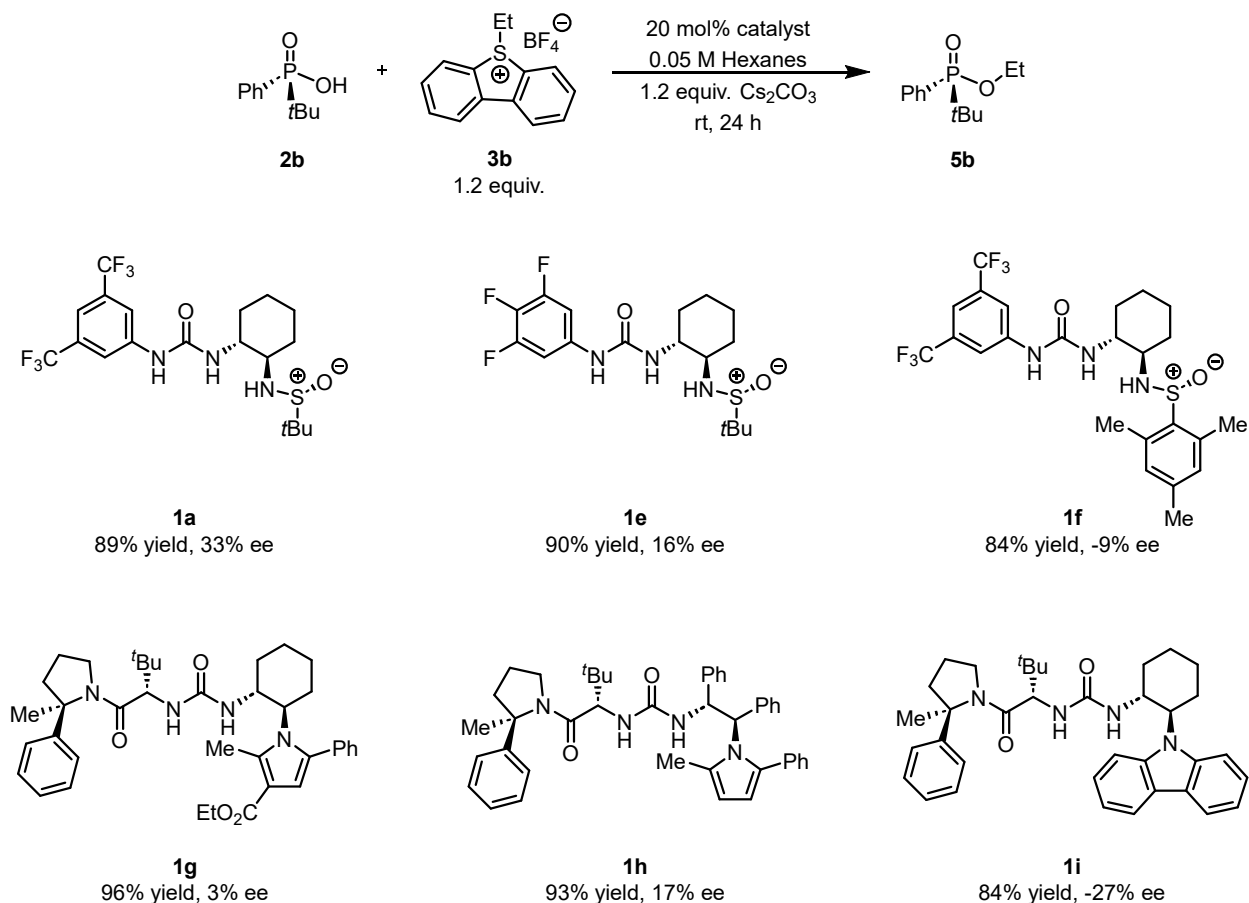
Figure 3.5 Studies investigating the effect of catalyst structure on enantioselectivity with substrate 2b . Experiments were run on 0.05 mmol scale. Yield values reflect product quantification by 31 P NMR relative to an internal standard.
