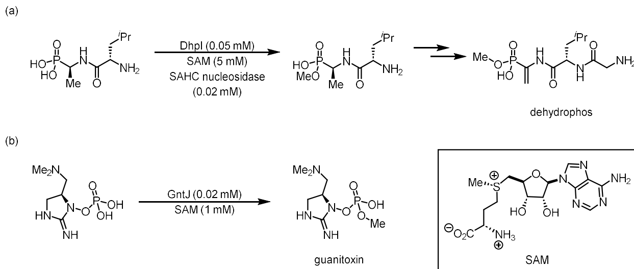
Figure 3.2 Biosynthetic examples of SAM-dependent methylation reactions of organophosphate intermediates catalyzed by O-methyltransferases.
