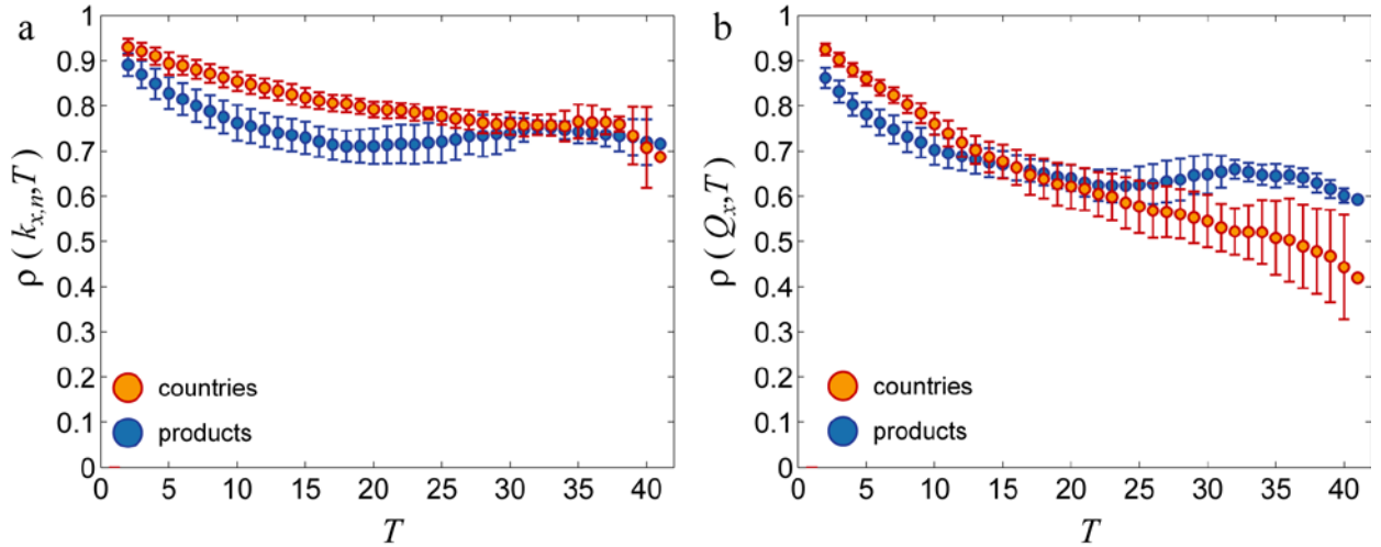
Figure 4 Changes in M_{cp} and in the Product Space. a. Average correlation between measures of economic complexity and product sophistication taken with a separation of T years ( n=19 ). b. Average correlation between the connectivity of countries and products in their respective projections of M_{cp} (the Country Space and the Product Space) measured T years apart.
