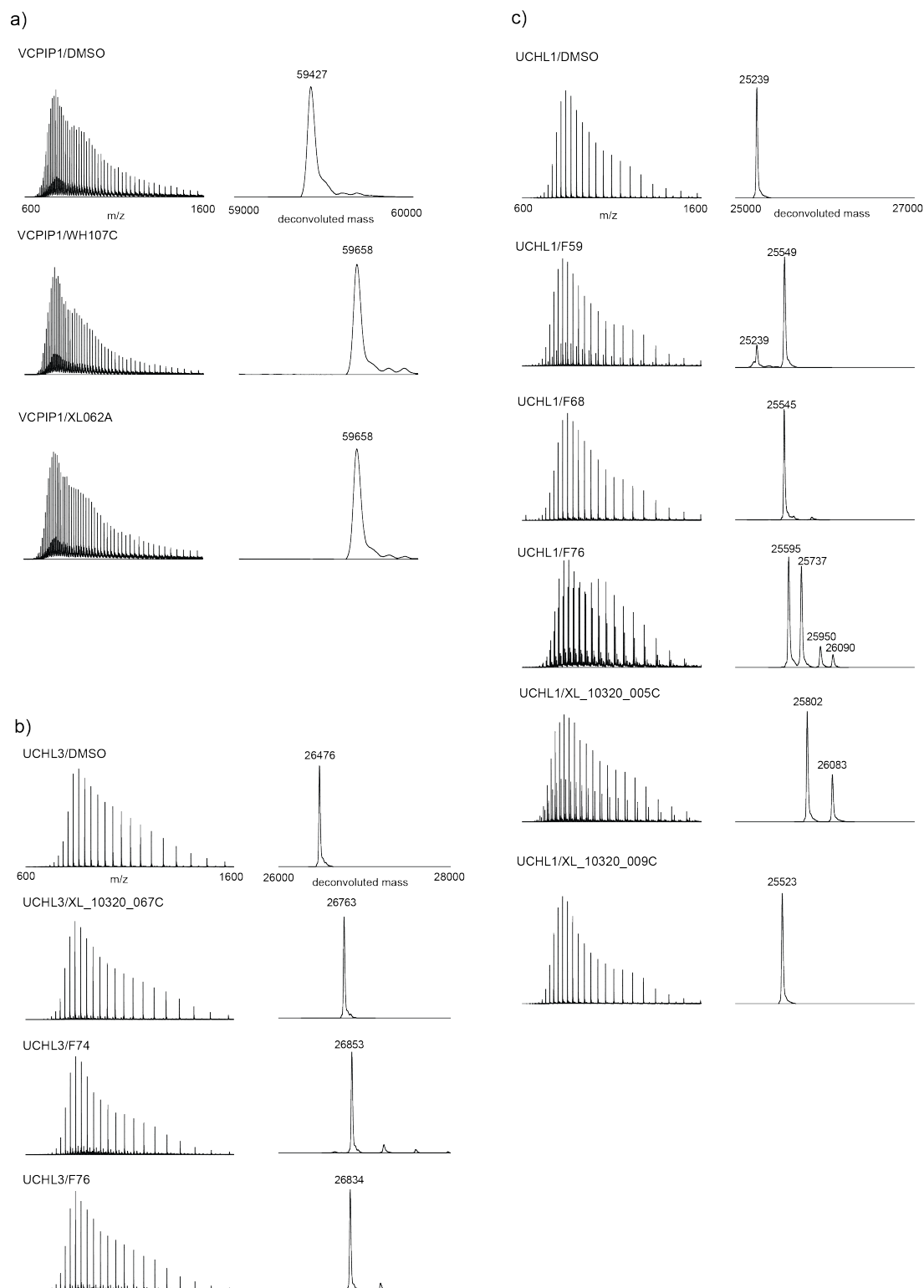
Figure 3.4. Intact protein MS validation. Purified a) VCPIP1, b) UCLH3, and c) UCLH1 protein were incubated with a 10x molar excess of compound and analyzed by LC-MS.
