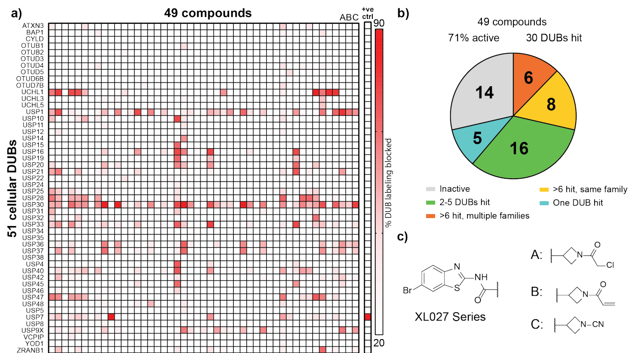
Figure 2.4. Pilot screen. a) Heatmap showing binding data for 49 compounds against 50 total endogenous DUBs. b) Library compounds displayed a wide range of activity against DUBs. c) The XL027 series highlighted how diversification at one part of the molecule can attenuate the DUB inhibition profile of resultant compounds.
