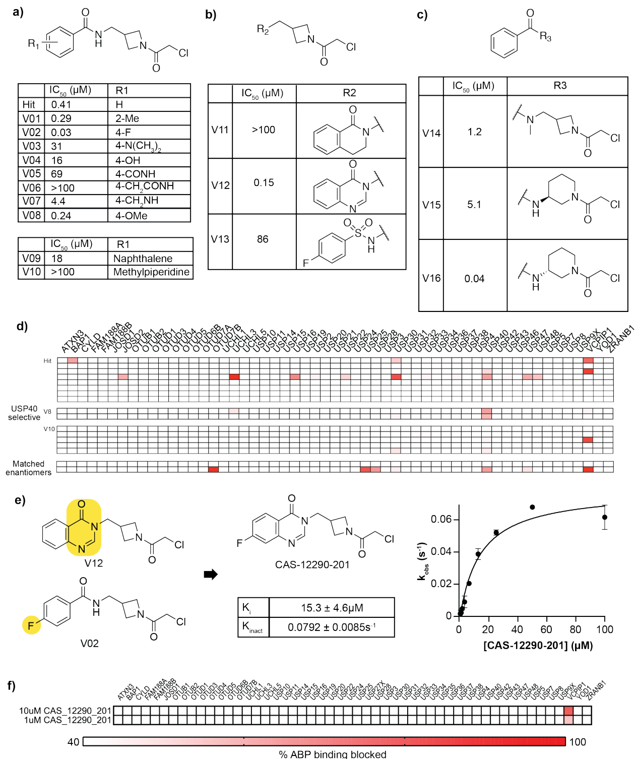
Figure 3.7. Target/target-class VCP1P1 inhibitor development. a-c) Biochemical IC 50 values and structures for the azetidinyl chloroacetamide focused mini-library. d) ABPP results for the mini-library compounds. e) Productive changes were combined to yield CAS-12290-201, novel potent
