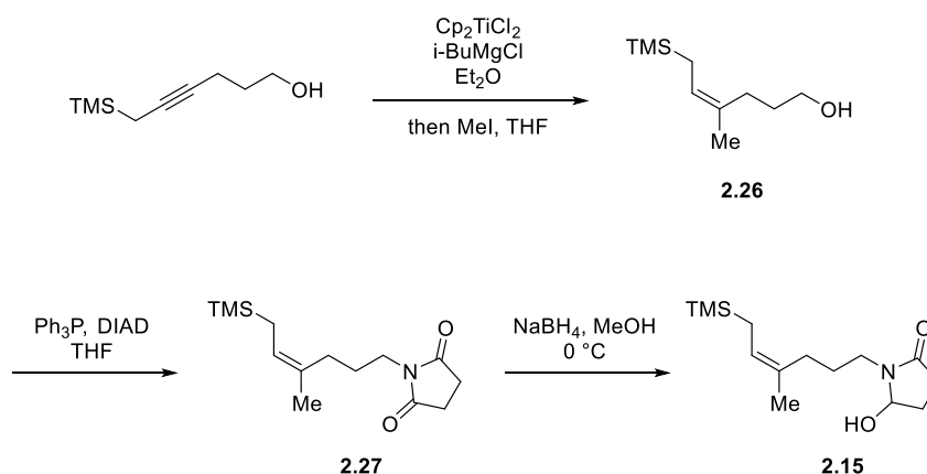
Scheme 2.9. Synthesis of 2.15
