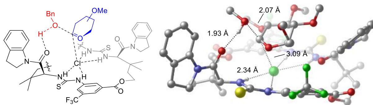
Figure 1.3. M06-2X/6-31g(d)/PCM transition structure for glycosylation (distances in Å).
