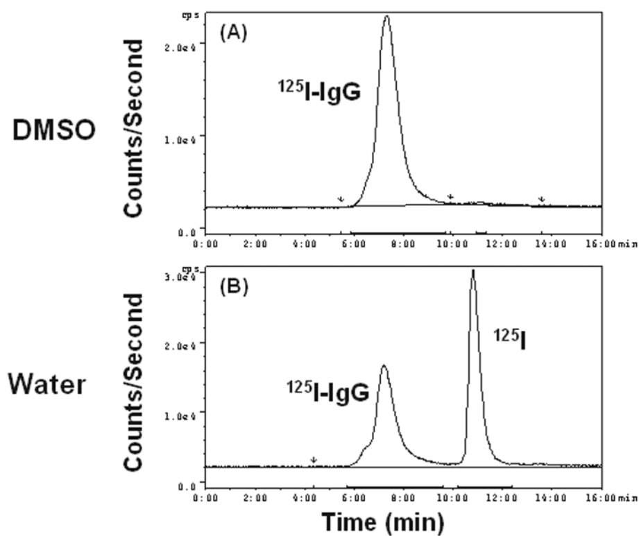
Fig. 6. HPLC of ^{125}\text{I} -IgG synthesized with 2 \mu\text{L} DMSO solution (20 \mu\text{g} IgG) or 4 \mu\text{L} water solution (20 \mu\text{g} IgG): (A) DMSO, yield 99.7%; (B) water, yield 49.5%.
