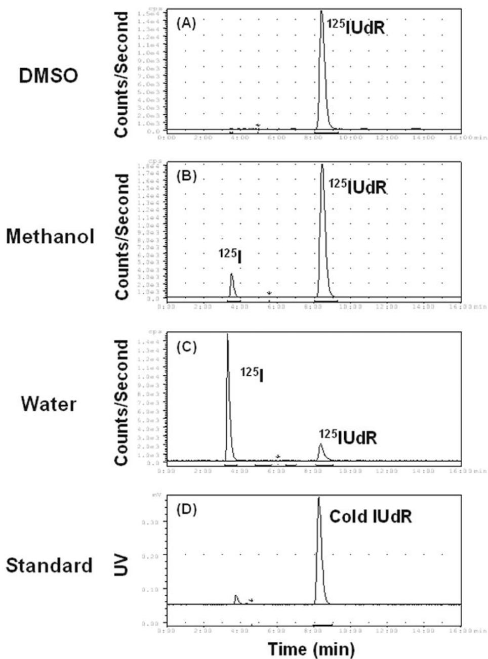
Fig. 1. HPLC of ^{125}\text{I} UdR synthesized with 1 \mu\text{L} precursor (1 \mu\text{g} SnUdR/ \mu\text{L} solvent): (A) DMSO, yield 99.8%; (B) methanol, yield 90.5%; (C) water, yield 82.1%; (D) standard.
