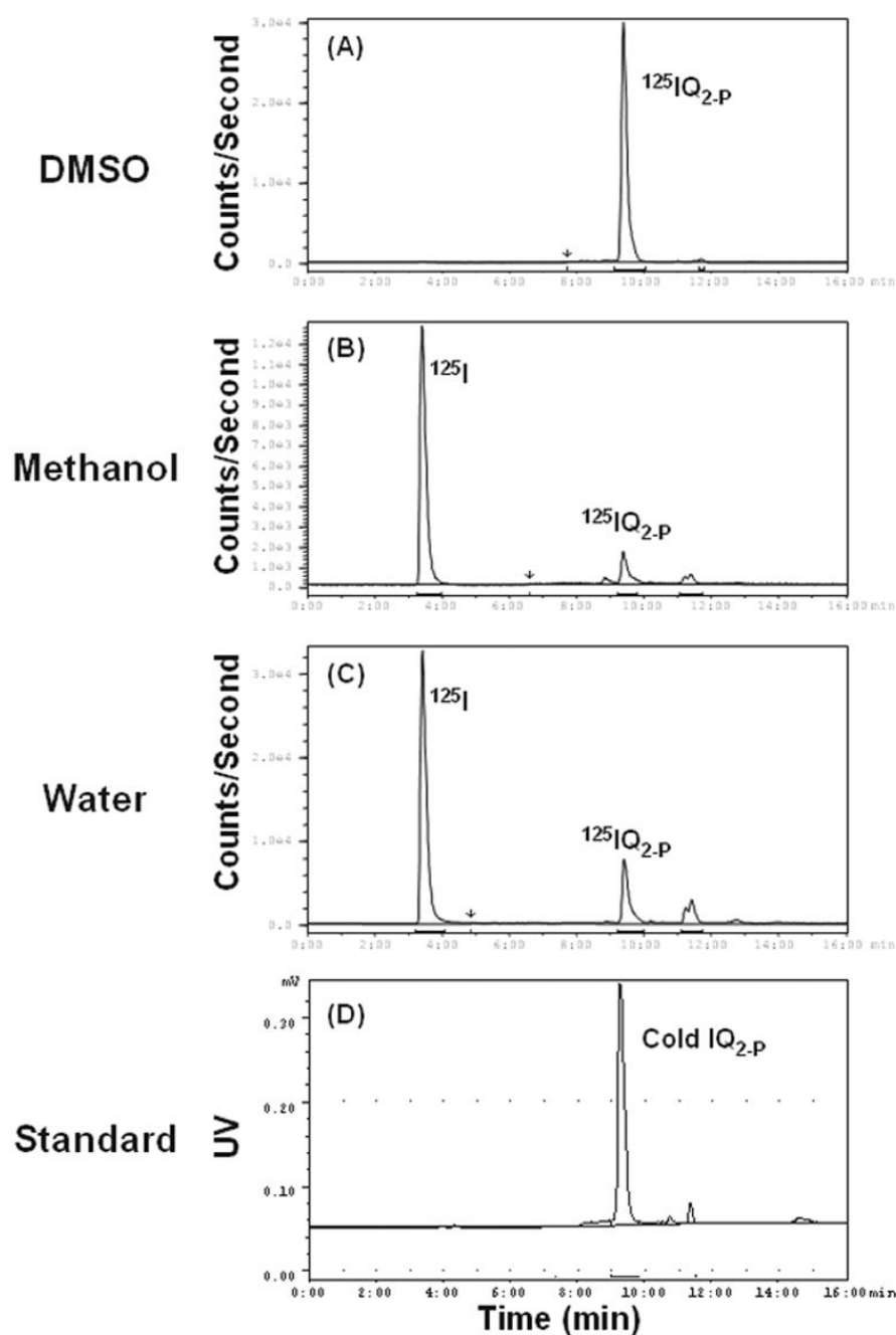
Fig. 2. HPLC of ^{125}\text{I} -Q 2 -p synthesized with 1 \mu\text{L} precursor (1 \mu\text{g} SnQ 2 -p/ \mu\text{L} solvent): (A) DMSO, yield 99.3%; (B) methanol, yield 11.6%; (C) water, yield 8.8%; (D) standard.
