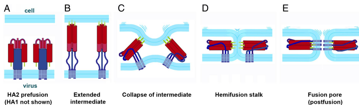
Fig. 1. Proposed mechanism for viral fusion proteins. (A) In the prefusion state, the protein, anchored in the viral membrane by a C-terminal transmembrane segment, folds so that the fusion peptide (green) is sequestered. (B) A ligand-dependent trigger (e.g., proton binding, for HA and many other viral fusion proteins) induces a conformational change in which the fusion peptide projects toward the target membrane, forming an extended intermediate that bridges the two membranes. (C) The intermediate collapses, by zipping up of the C-terminal part of the ectodomain (blue) alongside the trimer-clustered N-terminal part (red). (D) The collapse pulls the two membranes together, leading to formation of a hemifusion stalk. (E) A fusion pore opens up, and snapping into place of the membrane-proximal and transmembrane segments of the protein completes the conformational transition and stabilizes the fusion pore. (Figure adapted from ref. 40.)
