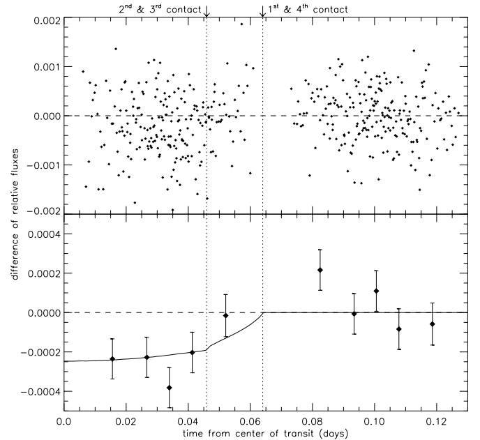
FIG. 4.—Top: Unbinned time series n_{\text{Na}} (Fig. 2, top panel). Bottom: These data binned in time (each point is the median value in each bin). There are 10 bins, with roughly equal numbers of observations per bin (42). The error bars indicate the estimated standard deviation of the median. The solid curve is a model for the difference of two transit curves (described in § 3), scaled to the observed offset in the mean during transit, \Delta n_{\text{Na}} = -2.32 \times 10^{-4} .
