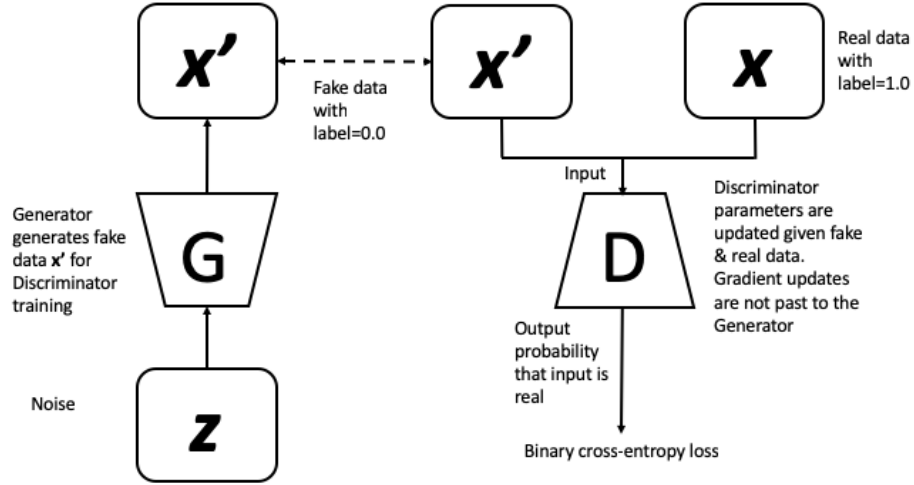
Figure 6.2: Training the discriminator is similar to training a binary classifier network using binary cross-entropy loss. The fake data is supplied by the generator while real data is from true samples.
