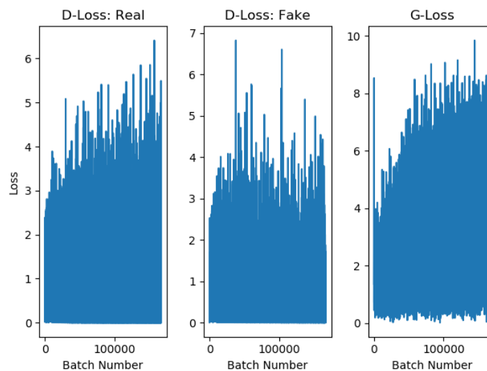
Figure 7.1: The discriminator and generator loss of the baseline DCGAN.
