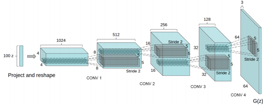
Figure 3.2: DCGAN generator used for LSUN scene modeling (Radford et al., 2015)
