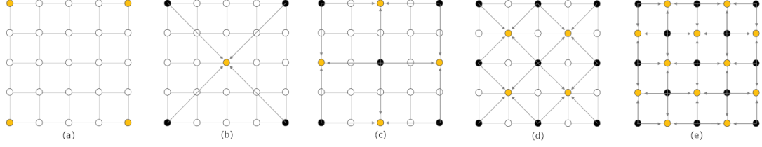
Figure 1.7: Steps involved in running the diamond-square algorithm on a 5 \times 5 array (Ewin, 2015).
