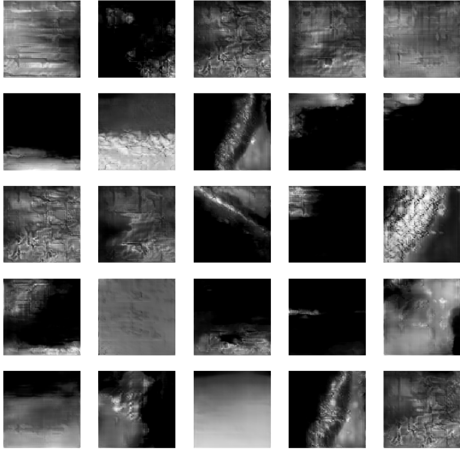
Figure 6.5: Randomly generated heightmap images from a trained DCGAN generator.
