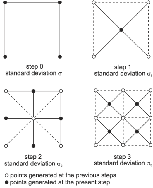
Figure 1.5: Iterations of Random Midpoint Displacement (Capasso, 2001).
