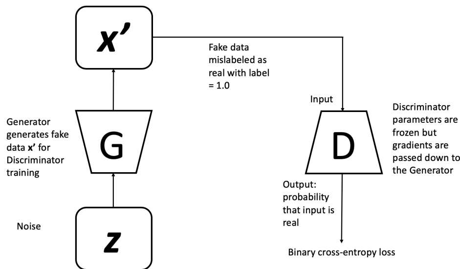
Figure 6.3: Training the generator is basically like any network using a binary cross-entropy loss function. The fake data from the generator is presented as genuine.
