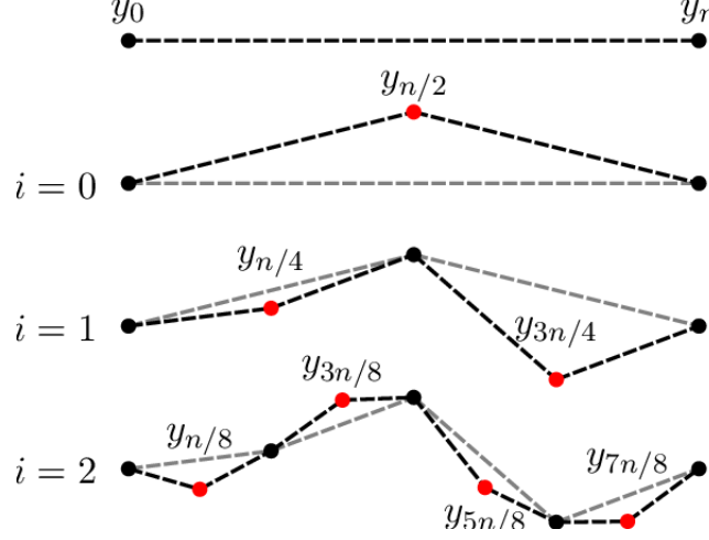
Figure 1.6: Random Midpoint Displacement applied to a line (Sund, 2014) using three iterations.
