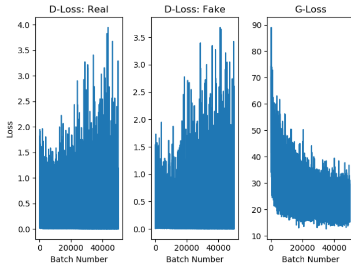
Figure 7.10: The discriminator and generator loss of the pix2pic GAN.
