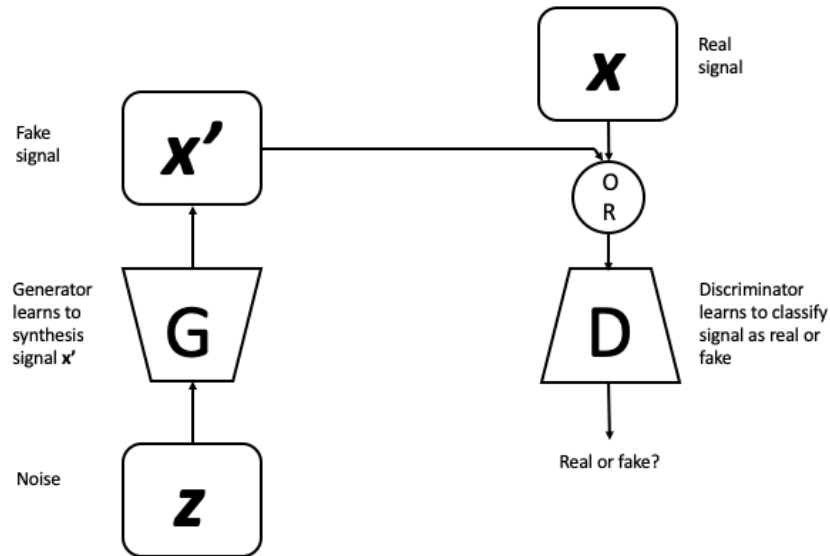
Figure 6.1: A GAN is made up of two networks, a generator, and a discriminator. The discriminator is trained to distinguish between real and fake signals or data. The generator's role is to generate fake signals or data that can eventually fool the discriminator.
