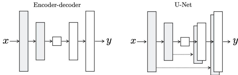
Figure 3.3: U-Net features an Encoder-decoder structure with skip connections that link both sides of the architecture.
