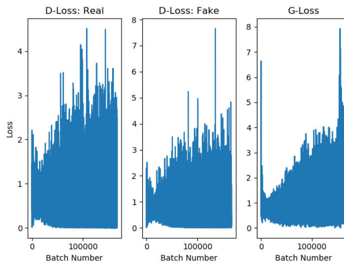
Figure 7.2: The discriminator and generator loss of the DCGAN with Gaussian noise.
