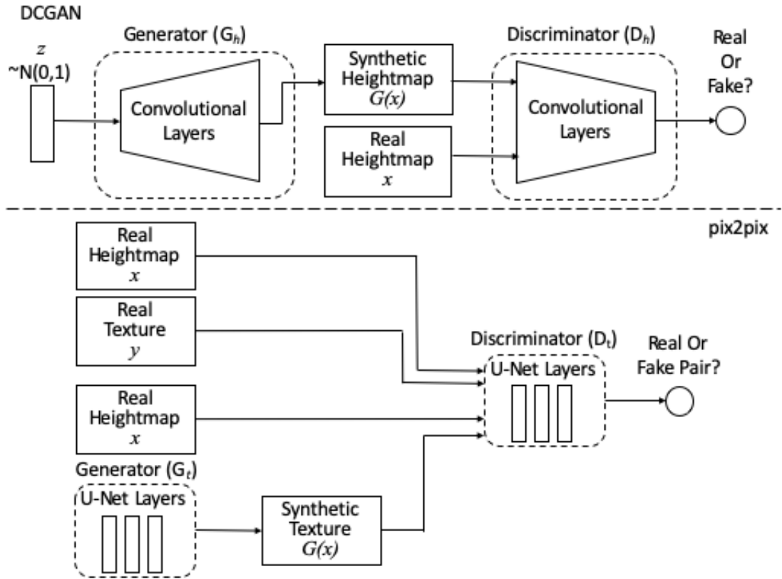
Figure 3.1: Two-stage GAN using DCGAN and pix2pix GAN.
