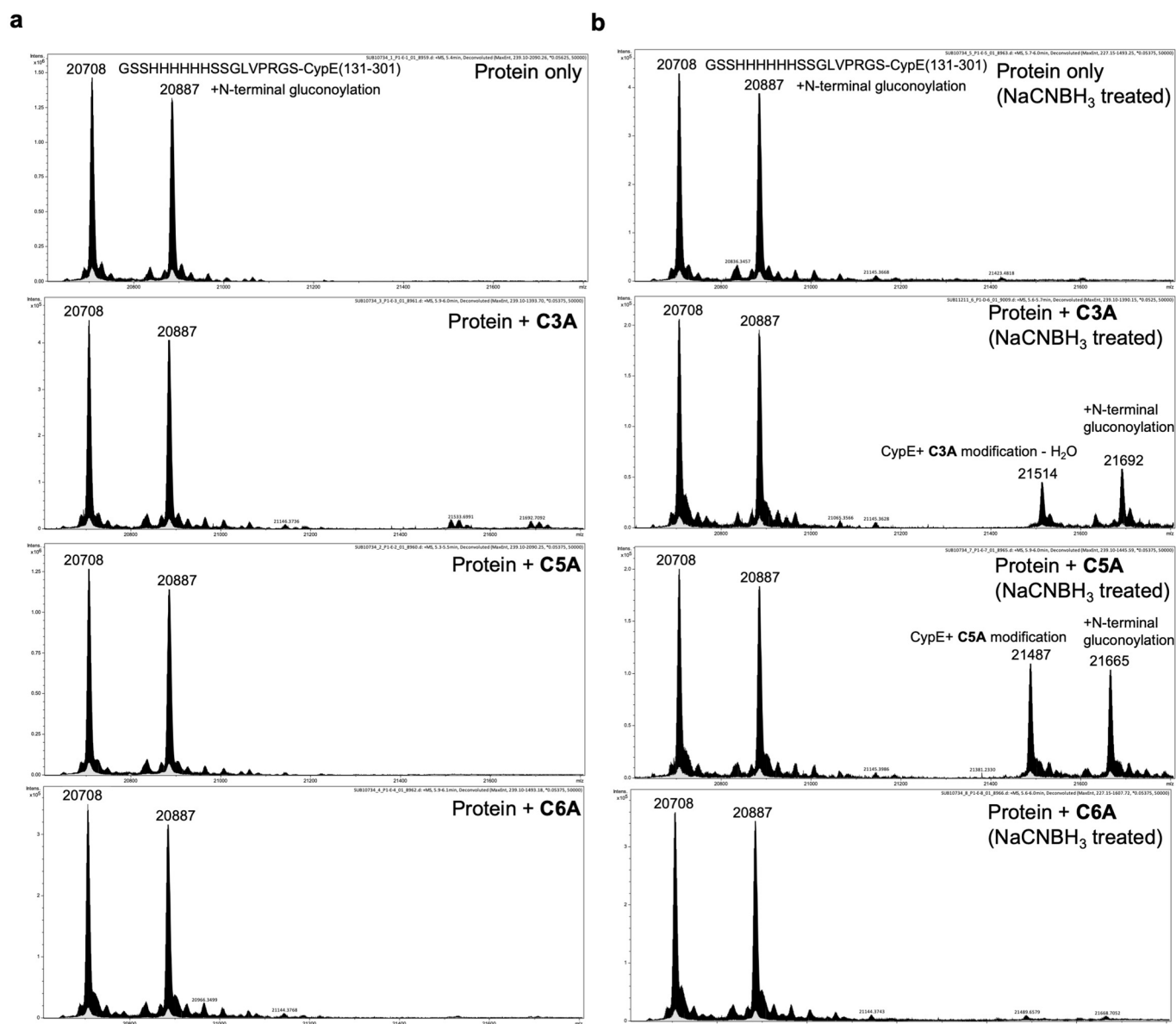
Extended Data Fig. 10 | Mass spectrometry analysis of compounds co-incubated with CypE. a, Mass spectrometry analysis of lysine covalent modification of CypE with C3A , C5A , and C6A . b, Mass spectrometry analysis of lysine covalent modification after treatment with NaCNBH 3 to trap the iminoboronate as a reduced lysine-linked secondary amine, highlighting relevant m/z regions. C3A and C5A show covalent modification (+779 Da and +806 Da, respectively) of CypE after reductive amination with NaCNBH 3 .
