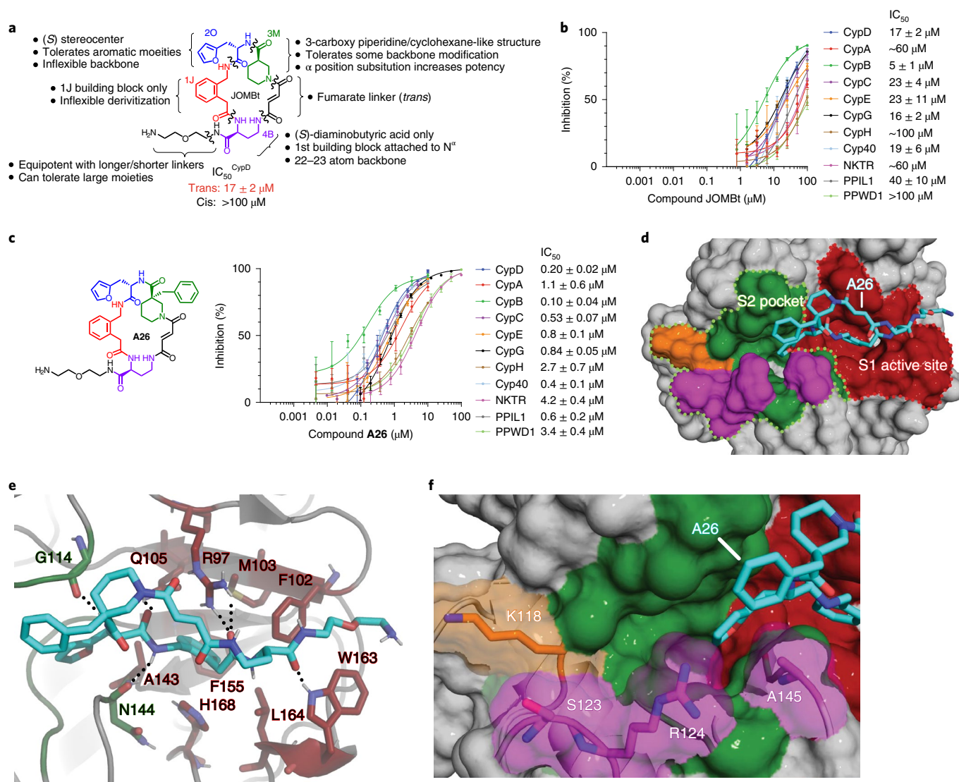
Fig. 1 | Selection of a DNA-templated library of 256,000 macrocycles for CypD affinity reveals novel cyclophilin inhibitors. a , Generalized trends in inhibition potency of CypD prolyl-isomerase activity from cyclophilin inhibition profiles of library hits and A -series macrocycles. b , JOMBt, showing weak and promiscuous cyclophilin inhibition of prolyl-isomerase activity. c , Compound A26 showing improved CypD potency but promiscuous inhibition. d , X-ray co-crystal structure of compound A26 (cyan) bound to CypD (PDB ID 7TGT , 1.06 Å resolution), shown as a space-filling model. A26 has a dual-binding mode involving the active site (red) and S2 pocket (green) of CypD. e , Active site binding interactions with A26 . The phenyl group provides the primary hydrophobic interactions with F102, M103, A143, F155, L164, and H168. Black dashes show predicted hydrogen bonding interactions with R97, Q105, G114, and W163 and the backbone of the A26 . f , S2 pocket binding pose of the furan of A26 , exhibiting a shallow interaction that does not engage non-conserved residues K118 (orange), S123 (magenta), and R124 (magenta) on the far side of the pocket. IC 50 values reflect mean \pm s.e.m. of three technical replicates. Data points and error bars reflect mean \pm s.d. of individual assays at one dose.
