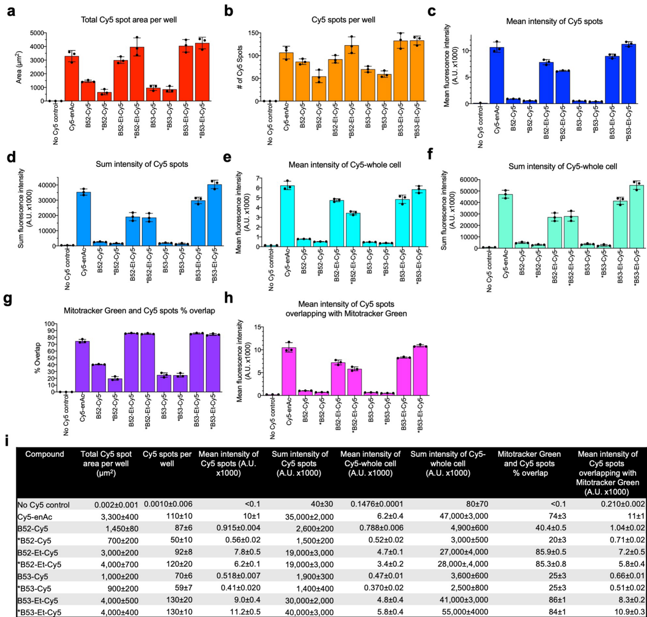
Extended Data Fig. 8 | Quantification of mitochondrial localization in HeLa cells by fluorescence microscopy of Cy5-conjugated compounds. HeLa cells were treated with Cy5-conjugated compounds and analyzed for a , total identifiable Cy5 spots; b , Cy5 spots per well; c , mean fluorescence intensity of identified Cy5 spots; d , sum of fluorescence intensity of identified Cy5 spots; e , mean Cy5 fluorescence intensity per cell; f , sum of Cy5 fluorescence in all measured cells; g , percent of Cy5 spots that overlap >70% with Mitotracker Green co-stain; and h , fluorescence intensity of Cy5 spots that overlap >70% with Mitotracker Green. i , values of data shown in a-h . Values and error bars reflect mean ± s.d. of three technical replicates.
