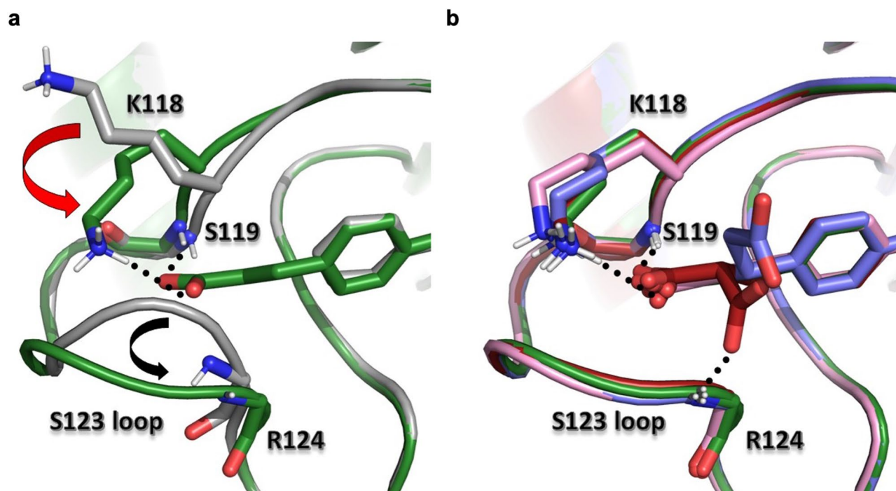
Extended Data Fig. 4 | Carboxylate-containing S2-binding moieties induce K118 side-chain and S123 backbone migration. a , Superposition of co-crystal structures of CypD with B2 (gray) and B23 (green). The side-chain of K118 typically is oriented away from the S2 pocket, as shown in co-crystal structures that do not contain carboxylate ligands, such as that of B2 . A properly placed carboxylate group ( B23 ) migrates K118's side-chain into the S2 pocket (red arrow), forming a salt bridge along with a hydrogen bond with S119's peptide backbone (black dashes). Also shown is the S123 loop migration that occurs when carboxylate-containing biphenyl groups bind deep into the S2 pocket (black arrow). b , Co-crystal structure superposition of CypD with B23 (green), B25 (pink), B52 (red) and B53 (purple). All properly placed carboxylate-containing ligands induce the same K118 and S123 conformational change. Dicarboxylates such as B52 and B53 also present the second carboxylate towards the S123 gatekeeper residue, the former exhibiting a hydrogen bond (black dashes) with the S123-R124 peptide backbone.
