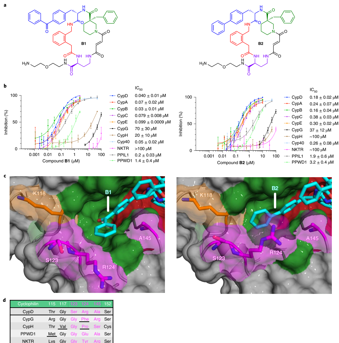
Fig. 2 | Compounds with large S2 pocket binding groups show reduced potency against cyclophilins with sterically occluded S2 pockets. a , Structure of B1 , B2 . b , Cyclophilin prolyl-isomerase inhibition screens for B1 and B2 . c , Co-crystal structures of B1 (PDB ID 7TGU, 1.21 Å resolution) or B2 (PDB ID 7TGV, 1.46 Å resolution) bound to CypD, viewing the S2 pocket. Active site binding is identical to that of A26 (Fig. 1e). d , Residues within the S2 pocket of cyclophilins inhibited less potently by B1 and B2 , with important residues underlined. The benzophenone or biphenyl group of B1 or B2 , respectively, fills the S2 pocket more completely, resulting in selectivity over cyclophilins with more sterically occluded or inflexible S2 pockets. CypD by contrast contains a relatively un-occluded S2 pocket and flexible R124 residue. IC_{50} values reflect mean \pm s.e.m. of three technical replicates. Data points and error bars reflect mean \pm s.d. of individual assays at one dose.
