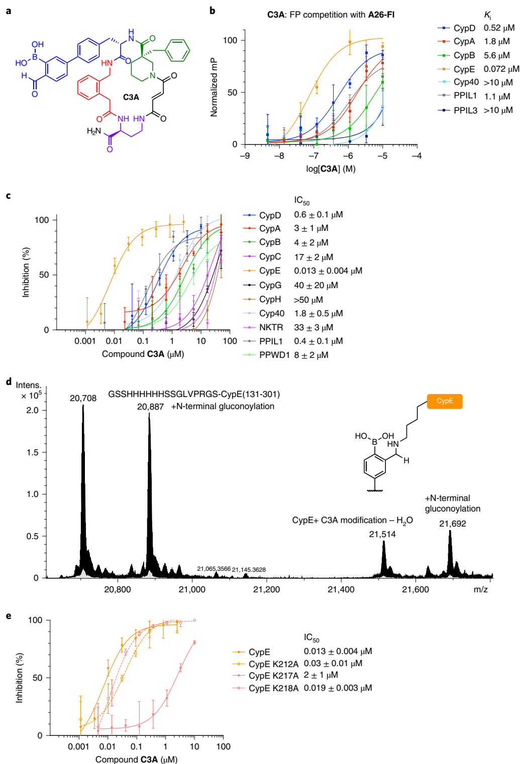
Fig. 6 | Aryl-carbonyl boronic acid C3A achieves selective inhibition of CypE. a , Structure of C3A. b , C3A fluorescence polarization (FP) competition with A26-Fl against cyclophilins with S2 pocket lysines. c , Cyclophilin prolyl-isomerase inhibition screen of C3A, showing potency and selectivity for CypE. d , Mass spectroscopy trace of CypE incubated with C3A and reduced with sodium cyanoborohydride. C3A shows an adduct consistent with CypE + amine-H 2 O (+806 Da), the result of iminoboronate formation followed by reductive amination. The mass of CypE is 20,708 Da, The CypE preparation also included N-terminal gluconoylation. e , Prolyl-isomerase inhibition by C3A against CypE S2 pocket lysine to alanine mutants. For the FP assay, the y-axis is normalized to internal control wells containing A26-Fl only (100%) and A26-Fl with cyclophilin (0%). Values reflect mean of three technical replicates and error bars reflect s.d. of individual assays at one dose. For the prolyl-isomerase assay in c and the CypE wild-type dose-response curve in e , IC_{50} values reflect mean \pm s.d. of four independent replicates (each comprising three technical replicates). Graph shows a representative single independent replicate (Independent replicate 3 is shown, containing three technical replicates) with data points and error bars reflecting mean \pm s.d. of individual assays at one dose. Further independent replicates are shown in Supplementary Fig. 28b. For the prolyl-isomerase assay in e , IC_{50} values for the CypE mutants reflect mean \pm s.e.m. of three technical replicates, while data points and error bars reflect mean \pm s.d. of individual assays at one dose.
