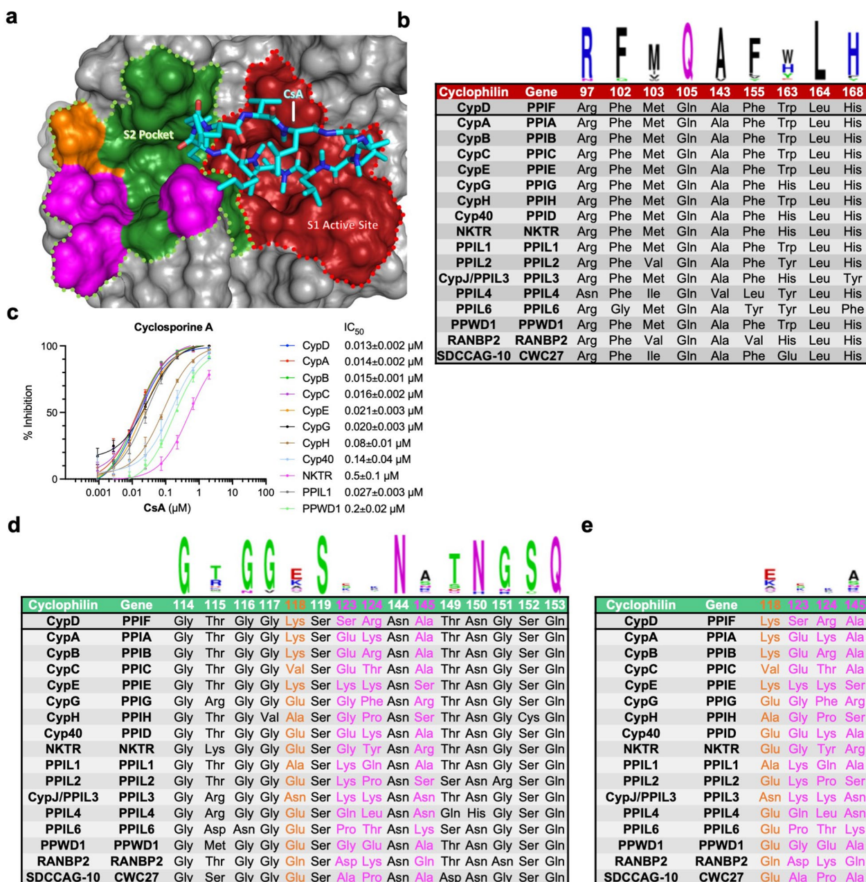
Extended Data Fig. 1 | Exclusive active site binding results in promiscuous cyclophilin inhibition. a , Co-crystal structure of CsA bound to CypD (PDB ID 2Z6W). CsA (cyan) binds to the active site (red) of CypD, a binding mode that does not engage more diversified residues that lie in the S2 pocket (green), including the primary gatekeepers (magenta) and the semiconserved K118 residue (orange). b , Active site (S1 pocket) residues with WebLogo plots, showing high conservation between the 17 cyclophilin isoforms with corresponding gene and protein identifier. c , Isomerization of the reporter peptide Suc-AAPF-AMC was measured with 5 nM cyclophilin and varying concentrations of CsA. CsA shows potent, but promiscuous inhibitory activity against all prolyl isomerase-active cyclophilins. Selective inhibition could rather be achieved through interactions with S2 pocket residues of cyclophilin subtypes ( d ). e , Cyclophilin S2 pocket residues that are the primary diversification sites within the active site-S2 pocket groove with WebLogo plots. Typical cyclophilin inhibitors such as CsA do not engage in interactions with these residues. All residue numbering is in reference to CypD. IC 50 values reflect mean \pm s.e.m. of three technical replicates. Data points and error bars reflect mean \pm s.d. of individual assays at one dose.
