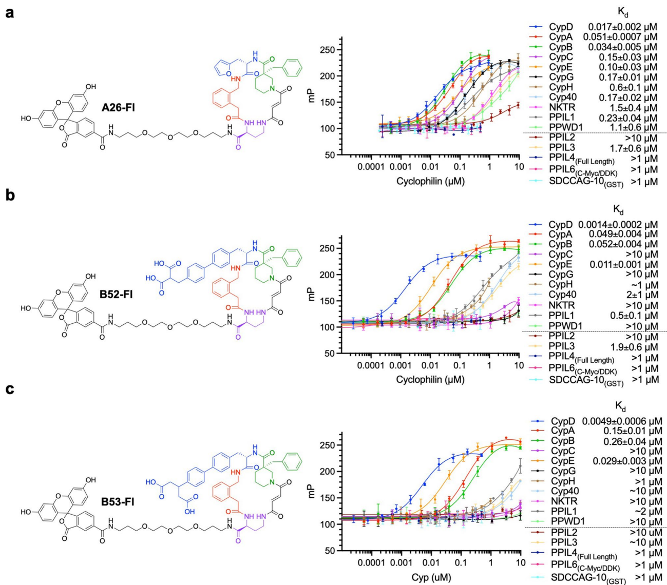
Extended Data Fig. 7 | Cyclophilin binding profiles using fluorescence polarization of fluorescein-labeled macrocycles. Each cyclophilin was titrated against 0.5 nM fluorescein-labeled macrocycle a , A26-FI; b , B52-FI; or c , B53-FI. Trends for selectivity follow those observed in the prolyl-isomerase assay. Cyclophilins in the legend below the dashed line are either prolyl-isomerase inactive or require much higher concentrations to observe prolyl isomerization in vitro . K_d values and error bars reflect mean ± s.e.m. of three technical replicates. Data points and error bars reflect mean ± s.d. of individual assays at one dose.
