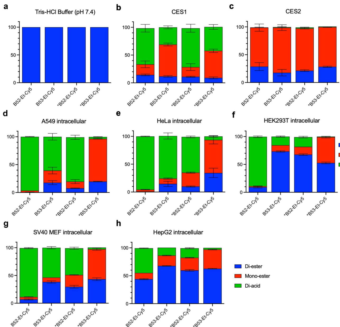
Extended Data Fig. 9 | Hydrolysis of ester prodrug CypD inhibitors. Compounds were evaluated for their ability to be hydrolyzed from di-ester to mono-ester, or to di-acid CypD inhibitors. Each reaction was analyzed by LC-MS, and ion abundances for each are shown as a percent of the total sum. These were conducted under conditions of: a , Tris-HCl buffer only; b , 250 nM carboxylesterase 1 (CES1); c , 250 nM carboxylesterase 2 (CES2); d , incubated with A549 cells for 48 h and intracellular fraction isolated; e , incubated with HeLa cells for 48 h and intracellular fraction isolated; f , incubated with HEK293T cells for 48 h and intracellular fraction isolated; g , incubated with MEFs for 48 h and intracellular fraction isolated; h , incubated with HepG2 cells for 36 h and intracellular fraction isolated. Esters show good stability in buffer and are only cleaved under esterase conditions, or intracellularly, with B52-Et-Cy5 showing the most rapidly hydrolyzed esters. Values and error bars reflect mean \pm s.d. of three technical replicates.
