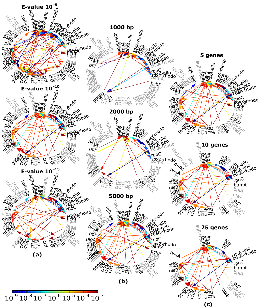
Figure 4.5: Associations between genes under varying parameters in the 7-m sample. Unless labeled otherwise, all associations are between at least 5 genes identified with e-values of 10-10 on contigs with at least 5000 basepairs. Arrows indicate direction of association: A \rightarrow B implies if A is present, B will frequently be present also. (a) Varying e-value used for gene identification, (b) varying minimum contig size, and (c) varying minimum number of genes for identification. Gene names in black were found to have associations with other genes; names in gray have sufficient copy numbers for calculation under the criteria for that trial, but no associations; “blank” gene names did not appear frequently enough to be calculated.
