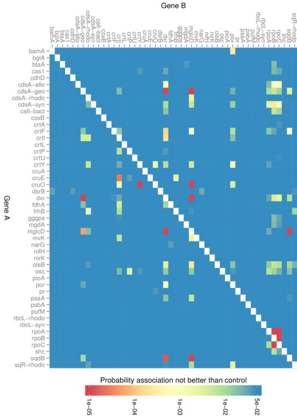
Figure 4.8: Heatmap showing associations between genes in lake bottom sediment with at least 5 copies, identified at e -value of 10-10, in contigs of length 5000 bp or greater. Linkages are directional from Gene A \rightarrow Gene B.
