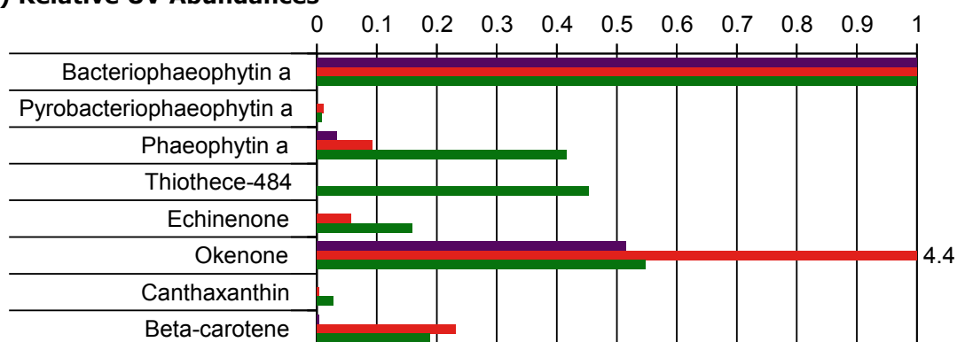
Figure 3.1. Relative abundances of carotenoids and chlorophyll derivatives from acetone extracts: (a) extracted MS ion data, (b) MRM transition data, and (c) UV-visible data. All values are reported as ratios relative to bacteriopheophytin a.
