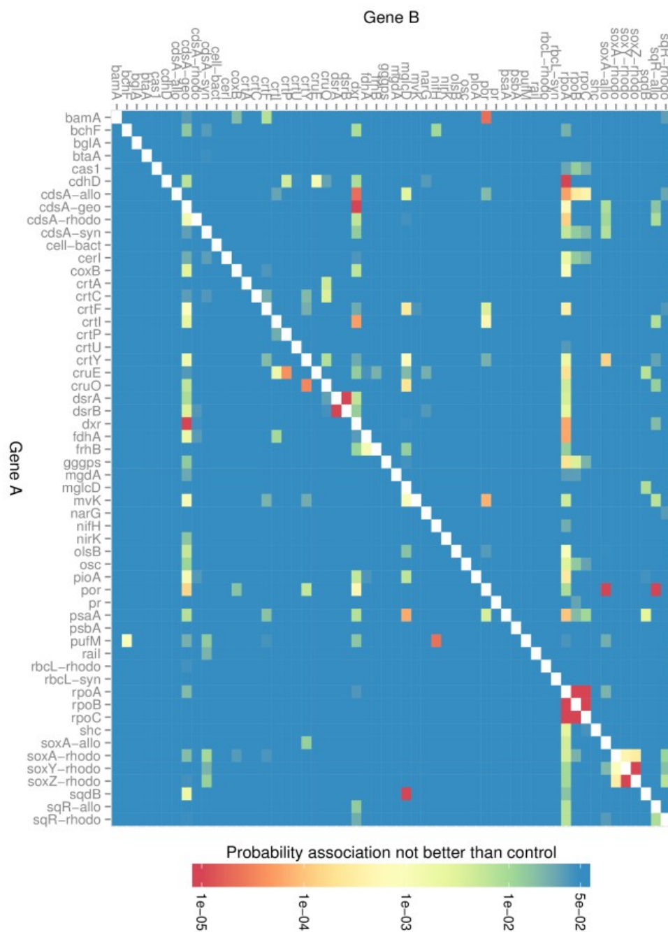
Figure 4.6: Heatmap showing associations between genes at 7-m with at least 5 copies, identified at E-value of 10-10, in contigs of length 5000 bp or greater. Linkages are directional from Gene A → Gene B.
