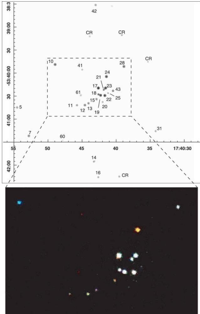
FIG. 1.— Top : Finding chart for sources detected with WAVDETECT in medium band (0.5–4.5 keV), with four probable cosmic-ray events (all counts recorded within \lesssim 30 s) marked. Bottom : X-ray color image constructed from soft (0.5–1.2 keV; red), medium (1.2–2 keV; green), and hard (2–6 keV; blue) bands for sources detected with Chandra in the central \sim 1' in NGC 6397. The cluster center is within \sim 1'' of U19 (CV2).
