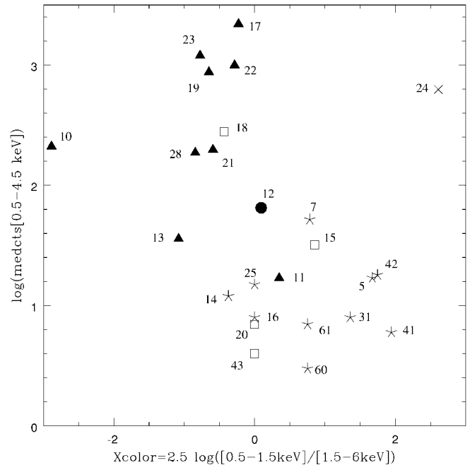
FIG. 2.—X-ray color-magnitude diagram, with probable source types labeled (as in GHE01): cross: qLMBX; filled circle: MSP; filled triangles: CV; open squares: BY Dra; five-point stars: unidentified. Source numbers correspond to those in Table 1.
