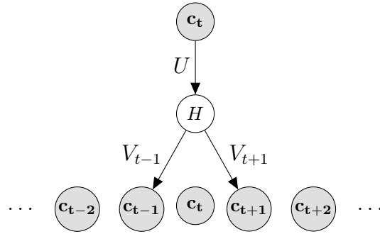
Figure 3.3: Skipgram neural network with window size w = 1 .
