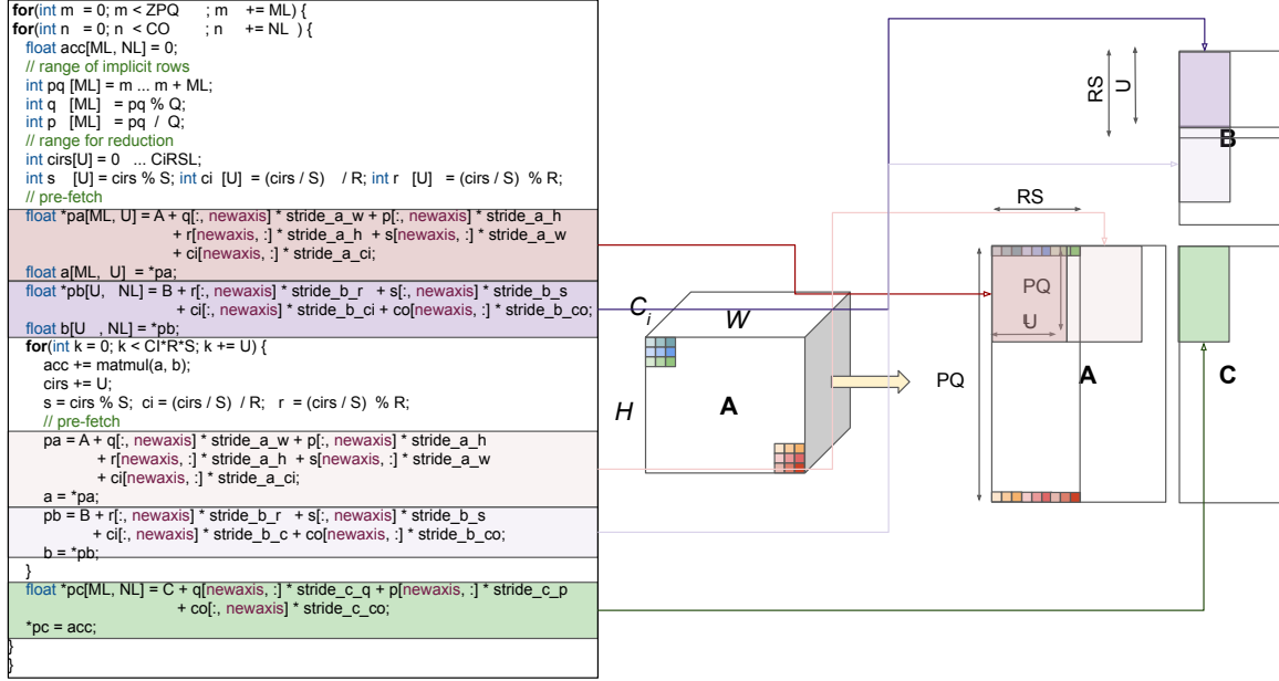
Figure 4.4: Blocked algorithm for dense convolutions. For simplicity, we assume N = 1 .
