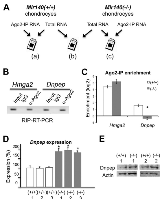
FIG. 6. miR-140 targets Dnpep in mouse chondrocytes. (A) Experimental strategy. RNA was prepared from the Ago2-IP fraction and total RNA from wild-type and Mir140 -null primary chondrocytes and subjected to expression profiling. RNA enriched in the Ago2-IP fraction was first identified in wild-type (a) and Mir140 -null (c) chondrocytes; genes that were enriched in the Ago2-IP fraction in wild-type but not in Mir140 -null chondrocytes were selected. Among them, those upregulated in Mir140 -null chondrocytes (b) were subjected to further investigation. (B) RNA immunoprecipitation followed by RT-PCR (RIP-RT-PCR) shows the specific association between Hmga2 and Dnpep transcripts and Ago2 in wild-type cells. (C) Dnpep is associated with Argonaute 2 (Ago2) in wild-type but not in Mir140 -null chondrocytes. Ago2 association was determined by comparing transcript levels of Ago2 immunoprecipitants with those of total RNA (Input in panel B). Transcript levels were expressed relative to that of GAPDH of each fraction. Ago2-IP enrichment ratios were calculated by dividing normalized transcript levels in the Ago2-IP RNA by those in total RNA. The relative enrichment of Dnpep in the Ago2-IP fraction is significantly less in Mir140 -null chondrocytes, whereas Hmga2 , a quintessential target of let-7 miRNAs, is enriched in the Ago2-IP fractions of both Mir140 -null and wild-type chondrocytes (*, P < 0.05 , n = 4 , t test). (D, E) Dnpep is upregulated in Mir140 -null primary rib chondrocytes both at the RNA level (D) and at the protein level (E).
