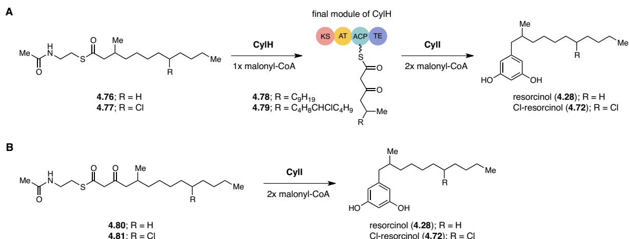
Scheme 4.13: In vitro assays of CylI and the final module of CylH using non-chlorinated or chlorinated substrates. A) Coupled CylH and CylI assays. B) CylI assay.
