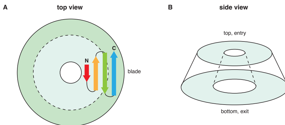
Figure 5.9: Diagram of a typical domain with \beta -propeller fold. A) Domains with a \beta -propeller fold has multiple blades that consist of a four-stranded antiparallel \beta -sheets. B) \beta -propeller protein forms a disc shape with a central tunnel.
