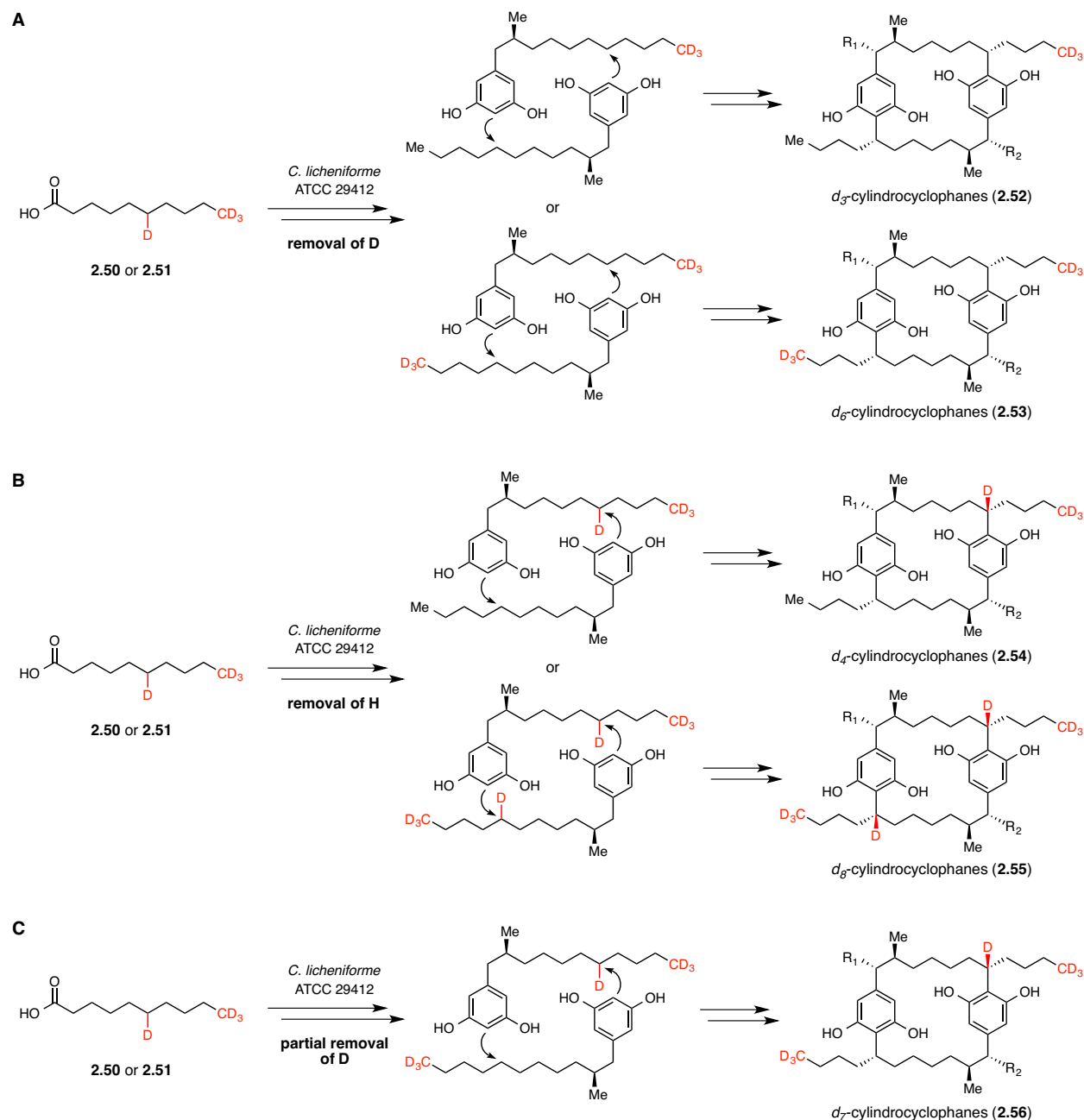
Scheme 2.19: Possible outcomes of the stereoselectively labeled decanoic acid feeding studies. A) Selective removal of deuterium results in the production of d 3 - and d 6 -cyclindrocyclophanes. B) Selective removal of hydrogen results in the production of d 4 - and d 8 -cyclindrocyclophanes. C) Partial removal of deuterium may lead to coupling of d 3 - and d 4 -labeled precursors to form d 7 -cyclindrocyclophanes.
