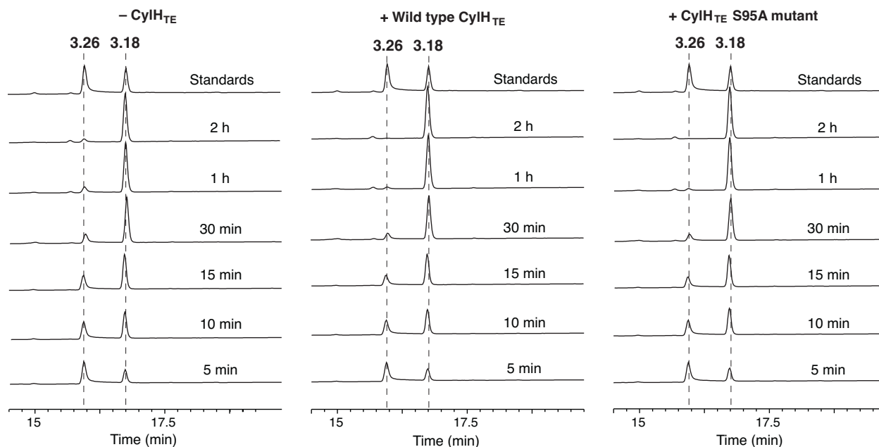
Figure 3.9: Time course analysis of the CylI assay with and without CylH TE or CylH TE -S95A (monitored at 230 nm).
