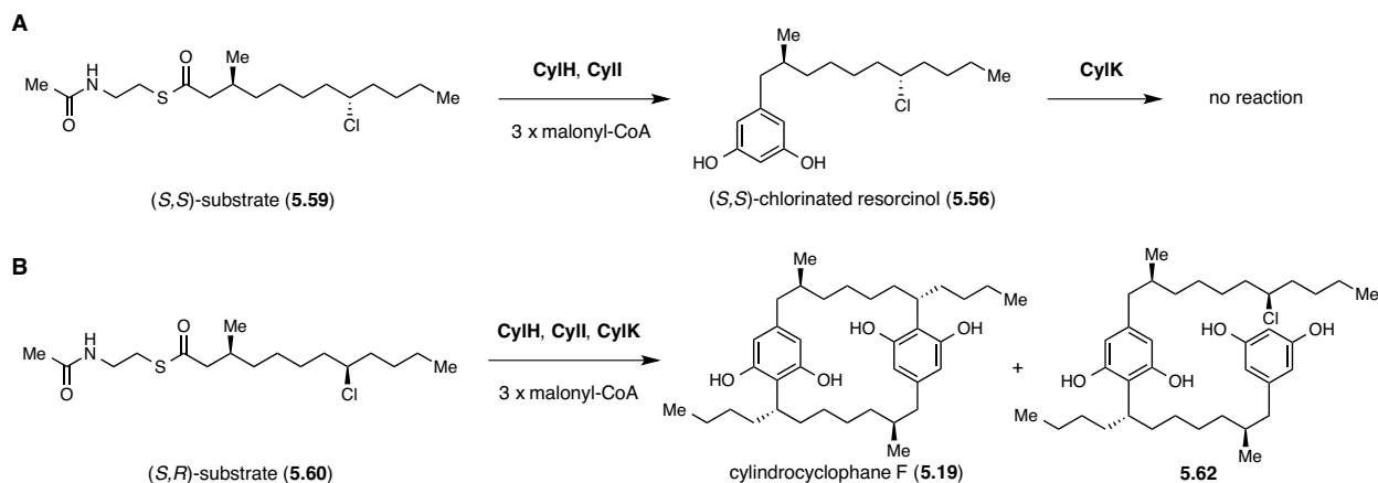
Scheme 5.12: Outcomes of the coupled CylH, CylI and CylK assays using diastereomerically-enriched substrates.
