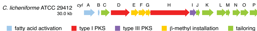
Figure 2.5: ORF diagram of the candidate cyl gene cluster.
