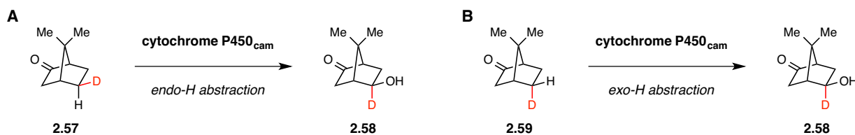
Scheme 2.20: Mechanistic studies of the cytochrome P450 camphor hydroxylase. 33 A) Deuterium labeling at the 5-exo position results in preferential abstraction of the 5-endo-hydrogen atom. The hydroxylation occurs at the 5-exo position, which results in the inversion of stereochemistry. B) Deuterium labeling at the 5-endo position results in preferential abstraction of the 5-exo-hydrogen atom and the stereochemistry is retained in the product.
