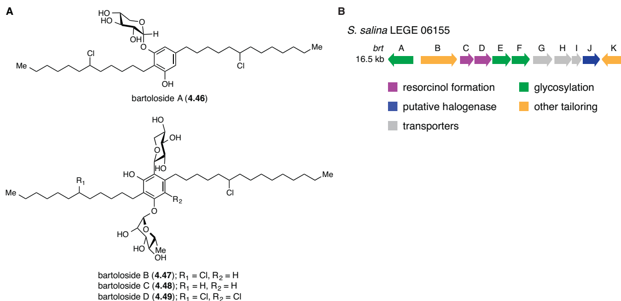
Figure 4.6: Discovery of the bartoloside ( brt ) biosynthetic gene cluster. A) Structures of the bartolosides. B) The brt gene cluster contains a CylC homolog, BrtJ.
