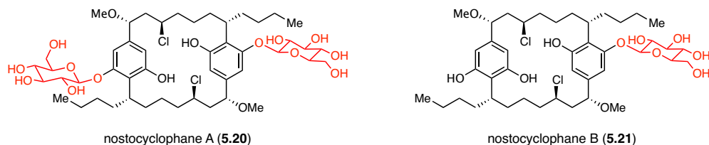
Figure 5.1: Structures of glycosylated nostocyclophanes A and B.
