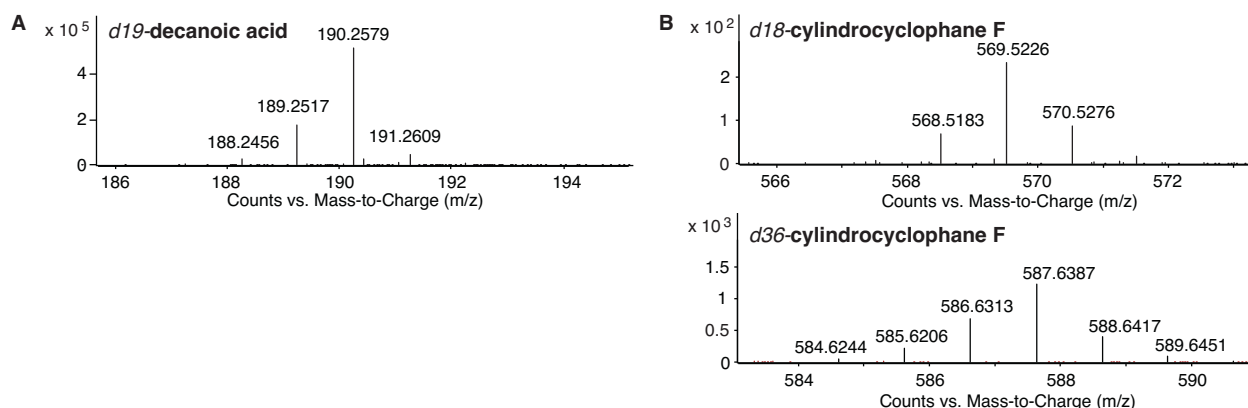
Figure 2.19: LC-MS m/z isotope distribution of deuterium labeled compounds in the feeding experiments. A) Isotope distribution of d_{19} -decanoic acid used for the feeding experiment. B) Isotope distribution of d_{18} - and d_{36} -cylindrocyclophane F detected in the feeding study samples.
