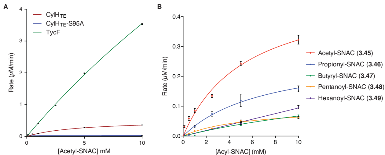
Figure 3.14: Michaelis-Menten curves from the spectrophotometric assays. A) Hydrolysis of acetyl-SNAC by CylH TE , CylH TE -S95A, and TycF performed in triplicate. B) Hydrolysis of acyl-SNAC substrates by CylH TE performed in duplicate.
