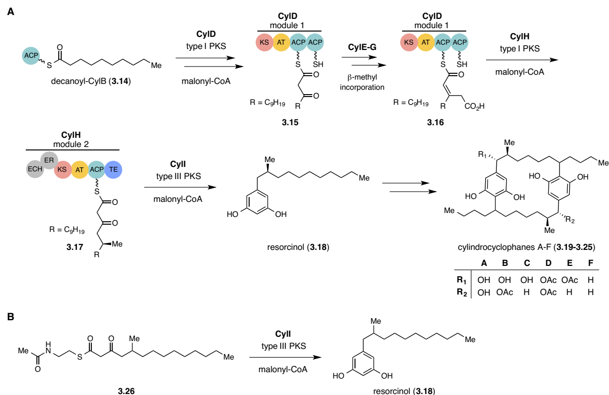
Scheme 3.7: Type I PKS assembly line termination in the cylindrocyclophane biosynthesis. A) The termination of the type I PKS assembly line appears to be catalyzed by the type III PKS CyII. B) In vitro CyII assay with the synthetic \alpha -ketoacyl-SNAC substrate leads to resorcinol formation.
