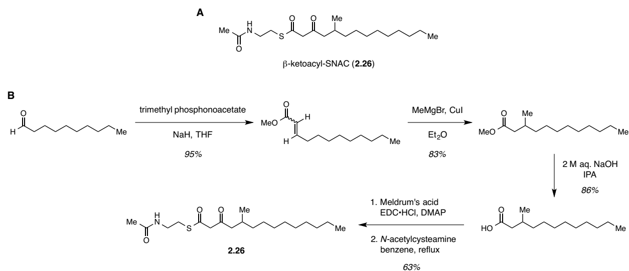
Figure 2.12: The synthesis of the CyIIH ACP-tethered \beta -ketothioester ( 2.17 ) analog for CyII assays. A) Structure of the \beta -ketoacyl-SNAC substrate 2.26 . B) Synthetic route for the \beta -ketoacyl-SNAC substrate 2.26 .
