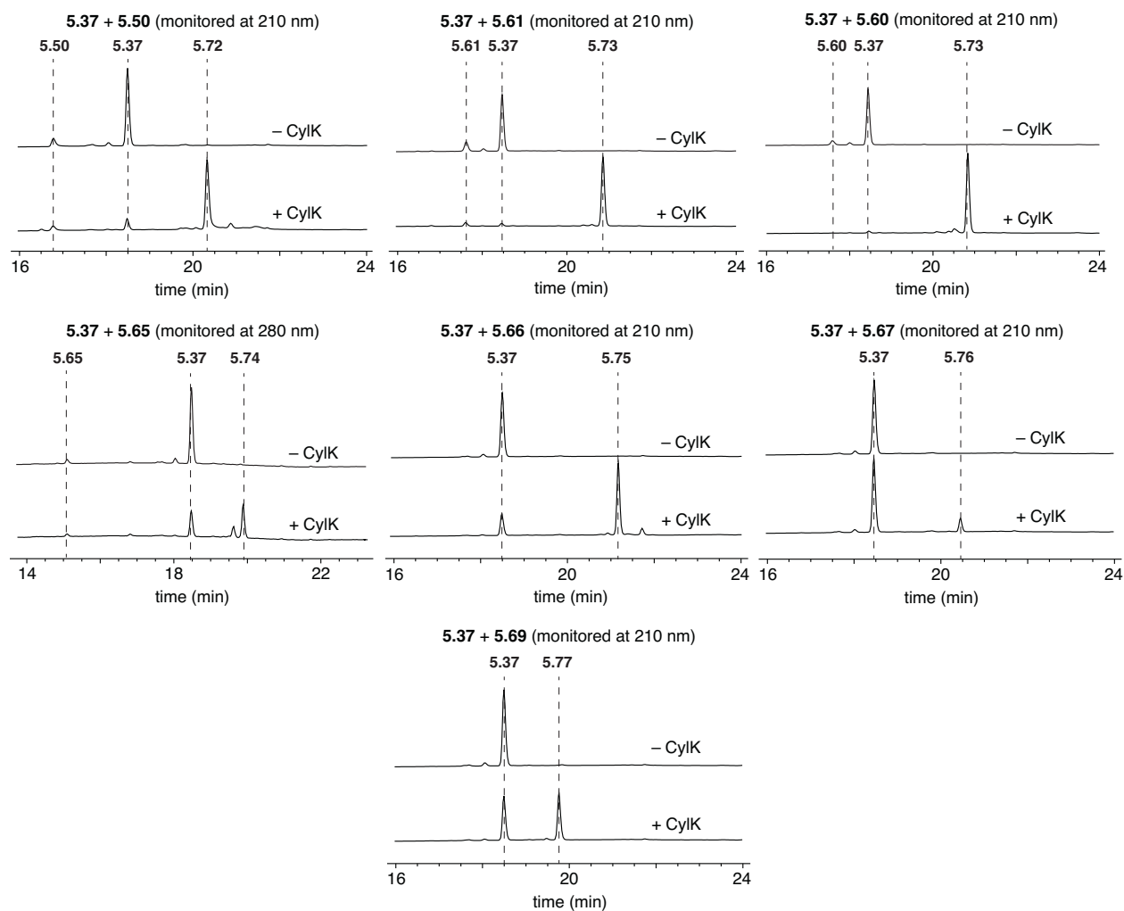
Figure 5.28: HPLC analysis of the CylK-catalyzed resorcinol alkylation assays with the product formation observed.
