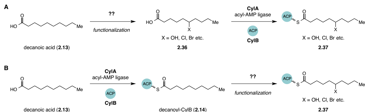
Scheme 2.16: Possible functionalization of the decanoic acid moiety early in the cylindrocyclophane biosynthesis.
