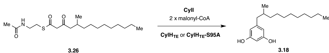
Scheme 3.10: Reaction used to examine the rate of resorcinol formation with and without the excised CylH TE .
