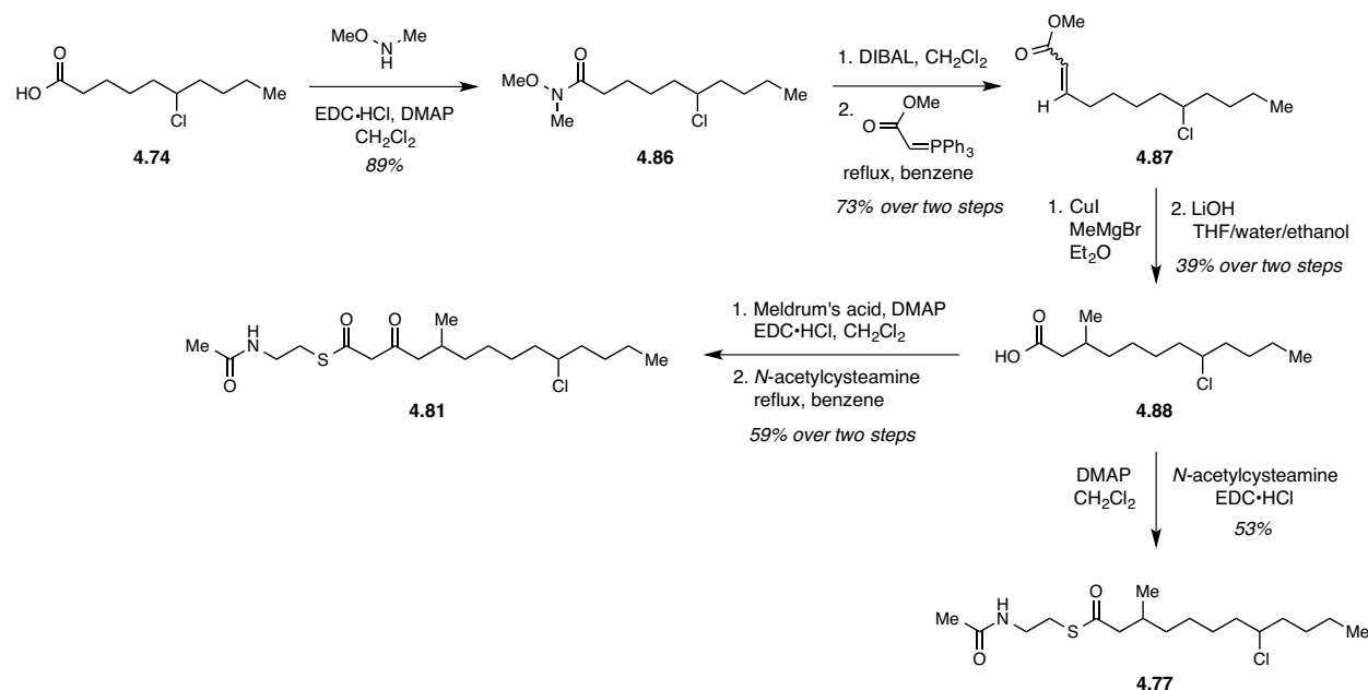
Scheme 4.16: Synthesis of chlorinated SNAC substrates for CylI and CylH PKS .
