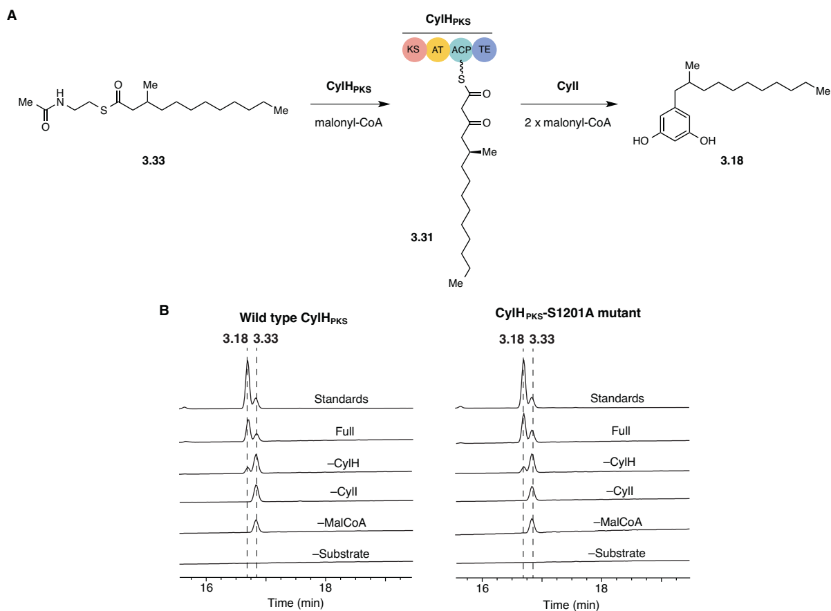
Figure 3.6: Coupled CylH PKS and CylI assay. A) CylH PKS forms \beta -ketoacyl-ACP 3.31 through elongation of the acyl-SNAC substrate 3.33 , and CylI uses 3.31 to form 3.18 . B) HPLC analysis of the coupled assays shows that resorcinol formation is observed with both CylH PKS and CylH PKS -S1201A mutant. Small amount of resorcinol formation is also seen in the control lacking CylH PKS due to the promiscuity of CylI (monitored at 210 nm).
