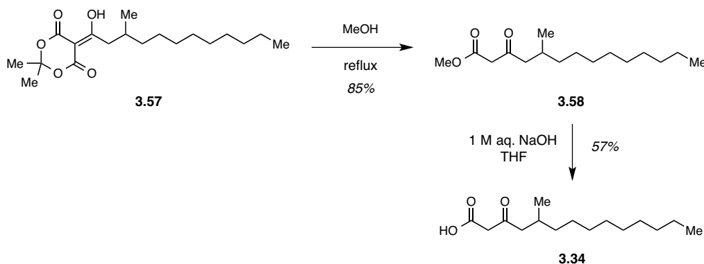
Scheme 3.15: Synthesis of the \beta -keto acid 3.34 as a product standard for CylH elongation assays.
