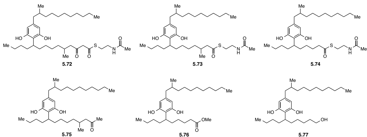
Figure 5.27: Predicted structures of the products of the CylK-catalyzed resorcinol alkylation assays in which product formation was observed.
