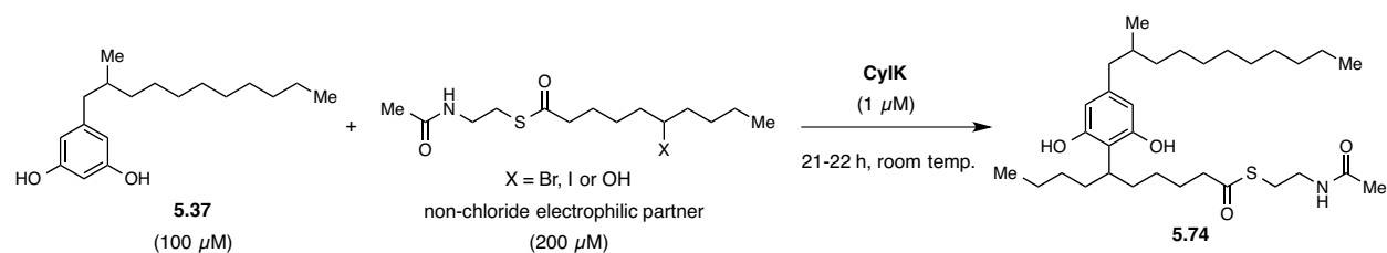
Scheme 5.18: CyLK assay with non-chloride electrophilic partners.
