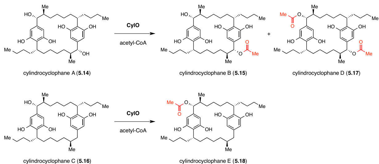
Scheme 5.4: Predicted acetyltransferase activity of CyIO to generate cylindrocyclophanes B, D and E.
