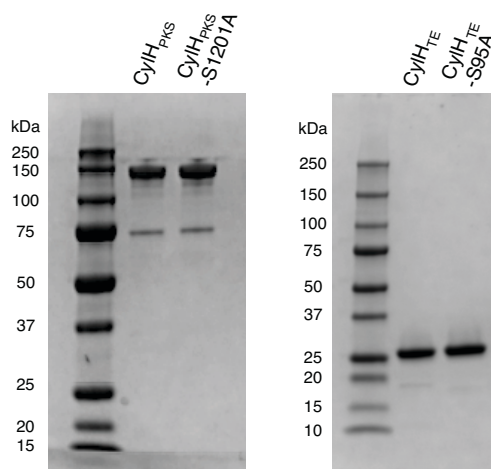
Figure 3.2: SDS-PAGE of purified C-His 6 -tagged CylH PKS and CylH PKS -S1201A (left), as well as CylH TE and CylH TE -S95A (right).
