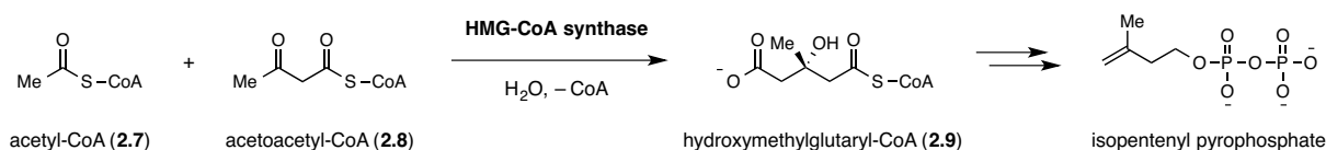
Scheme 2.1: Hydroxymethylglutaryl-CoA formation catalyzed by HMG-CoA synthase in isoprenoid biosynthesis.
