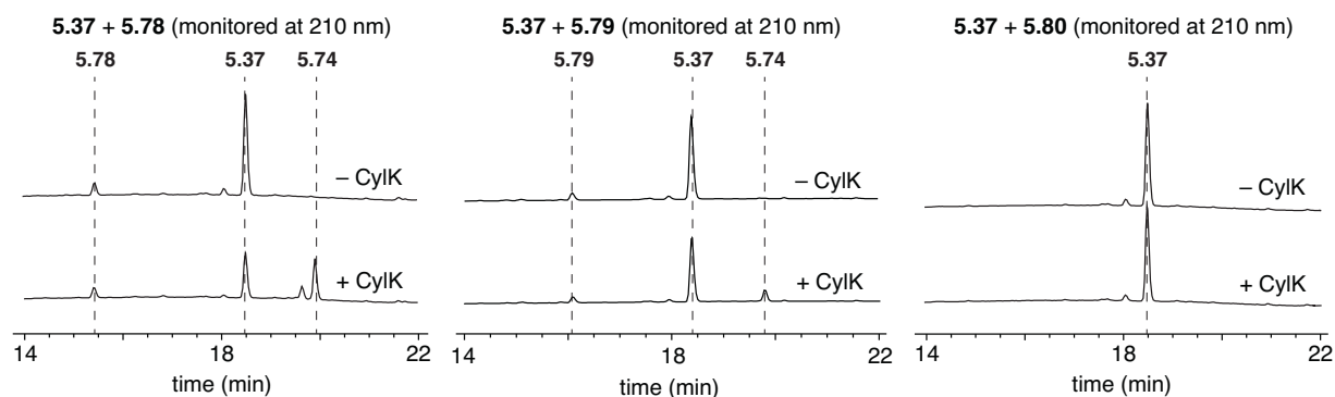
Figure 5.29: HPLC analysis of the CyLK-catalyzed resorcinol alkylation assays with non-chloride electrophiles.
