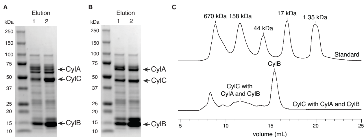
Figure 4.11: Co-expression of CylA, CylB and CylC. A) SDS-PAGE of purified N-His 6 -CylC and N-His 6 -CylB co-eluting with small amount of CylA. B) SDS-PAGE of untagged CylA and CylC co-eluting with N-His 6 -CylB. C) FPLC size exclusion chromatography of the co-purified CylA, CylB and CylC.
