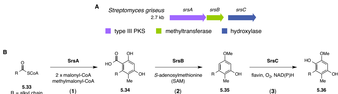
Figure 5.5: The production of alkylresorcinol methyl ethers by the srs gene cluster.
