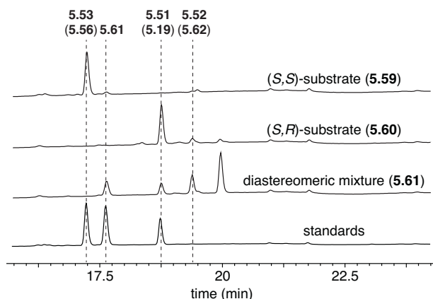
Figure 5.25: HPLC analysis of the coupled CylH, CylI and CylK assays (monitored at 230 nm).
