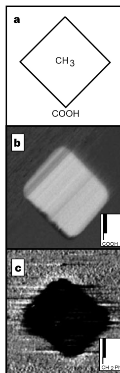
Figure 2. Chemically sensitive imaging with functionalized nanotube tips. a, Diagram of a patterned sample prepared by microcontact printing 19 and consisting of 10- \mu\text{m} squares of a methyl-terminated (hexadecanethiol) SAM region surrounded by a carboxylic acid-terminated (16-mercaptohexadecanoic acid) SAM background on gold. Tapping mode phase-lag images of the patterned sample in ethanol were recorded with b, an unmodified nanotube tip (COOH-terminated) and c, a benzylamine-functionalized nanotube tip (phenyl terminated). Darker regions indicate greater phase lag; the contrast in b and c corresponds to phase variations of 2.3^\circ and 2^\circ , respectively. The images are 16\text{ }\mu\text{m} \times 16\text{ }\mu\text{m} . Images and force curves were acquired with a Nanoscope III (Digital Instruments, Inc.). Imaging parameters were optimized for individual tips; typical ranges for the FESP (force modulation etched silicon probe) nanotube tips were (1) resonant frequencies, 28–33 kHz; (2) free r.m.s. oscillation amplitude, 30–90 nm, (3) set-point, 1–3 V, and (4) scan rate, 0.5–1.2 Hz.
