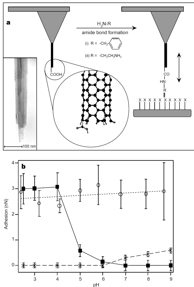
Figure 1. Preparation and characterization of functionalized carbon nanotube tips. a, Diagram illustrating the modification of a nanotube tip by coupling an amine ( \text{RNH}_2 ) to a pendant carboxyl group, and the application of this probe to sense specific interactions with functional groups (X) of a substrate. The circular inset is a molecular model of a single nanotube wall with one carboxyl group at the tip end. The multi-walled nanotubes used in our studies were attached to the pyramids of gold-coated Si cantilevers ( k = 0.5\text{--}5\text{ N m}^{-1} , Digital Instruments, Inc.) using an acrylic adhesive under the direct view of an optical microscope 5 . The as-made nanotube tips were shortened by applying a bias voltage between the tip and a sputtered Nb surface in an oxygen environment. Chemical modification of the nanotube ends was then carried out by placing a cantilever-tip assembly in a solution of 50 mM EDC (1-ethyl-3-(3-dimethylaminopropyl) carbodiimide hydrochloride) (Pierce) and 5 mM of either benzylamine or ethylenediamine in 0.1 M MES (2-[N-morpholino]ethanesulphonic acid) (Sigma) buffer pH 6.0, for 2 hours. The tips were then successively washed in 0.1 M solutions of MES, NaCl (Fisher) and deionized water. The nanotubes were prepared by arc-discharge and purified by oxidation (700 °C, air) until \sim 2\% of the original mass remained. Inset, TEM image showing the open end of a shortened nanotube tip. b, Adhesion force as a function of pH between the nanotube tips and a hydroxy-terminated SAM (11-thioundecanol on gold-coated mica): filled squares, carboxyl (unmodified); open circles, phenyl (modified with benzylamine); and crosses, amine (modified with ethylenediamine). Each data point corresponds to the mean of 50–100 adhesion measurements, and the error bars represent one standard deviation.
