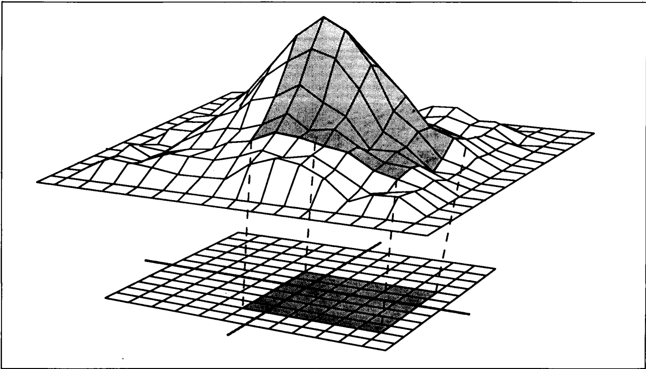
Figure 8. The selection of values from a subsection of the “master” (7 × 7) receptive field (above) to be used for individual input unit receptive field values (below). These are the fixed connection weights between points on the retina and a single input unit illustrated at the left of Figure 1.
