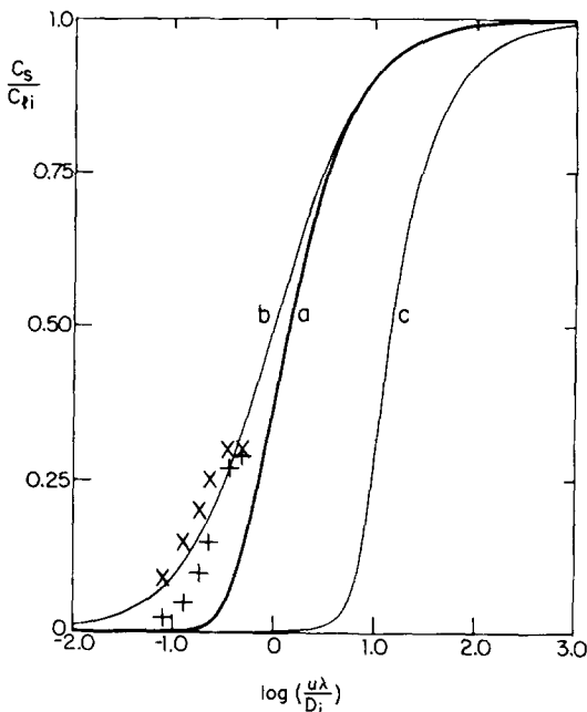
FIG. 4. Bismuth ( k_e = 7 \times 10^{-4} ) segregation in silicon. (a) stepwise growth model (this work), (b) continuous growth model (this work) and JGL, and (c) Baker model. 'x' — Baeri et al. data (111). '+' — Poate data (100). Data plotted assuming D_i/\lambda = D_L/\lambda = 10 m/s. Theoretical curves plotted assuming \alpha = 1 , T_i = T_M .
