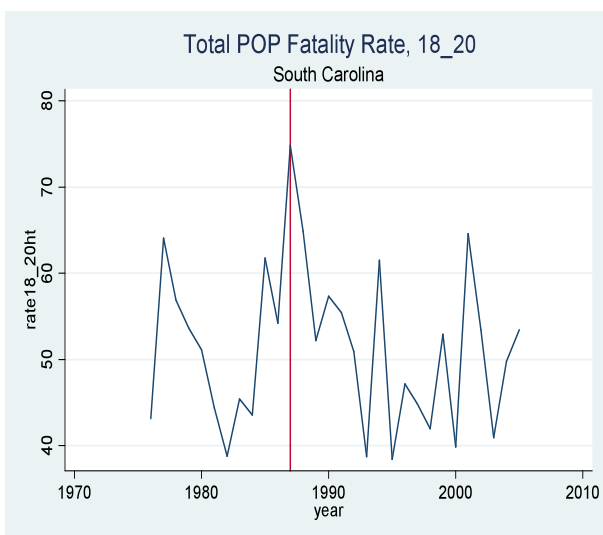
FIGURE 5: AVERAGE TOTAL FATALITY RATE PER 100,000 18-20 YEAR OLDS 1976-2005
