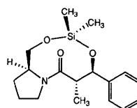
anti -Diastereomer (I)
