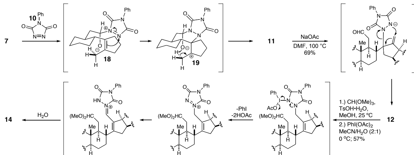
Scheme 3. Proposed mechanism of the selective aza-Prins reaction, [2,3]-sigmatropic rearrangement, and urazole oxidative hydrolysis
