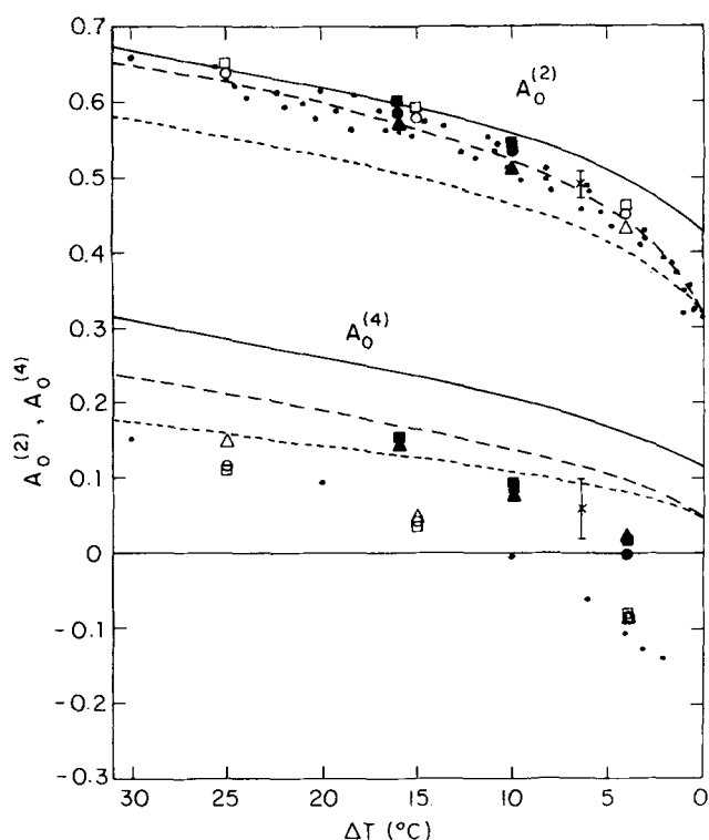
FIG. 18. Order parameters A_0^{(2)} and A_0^{(4)} deduced from the measurements on the 1576 (squares), 1597 (triangles), and the 1625 ( \circ ) \text{cm}^{-1} bands. The open data points are for the 20% mixture, and the closed data points for the neat MBBA. The cross is for the 10% mixture. Dots are data from Fig. 13. Solid lines: MS theory; dashed lines: HJL theory (---: m=10 ; ---: m=4 ; \lambda=-0.55 ).
