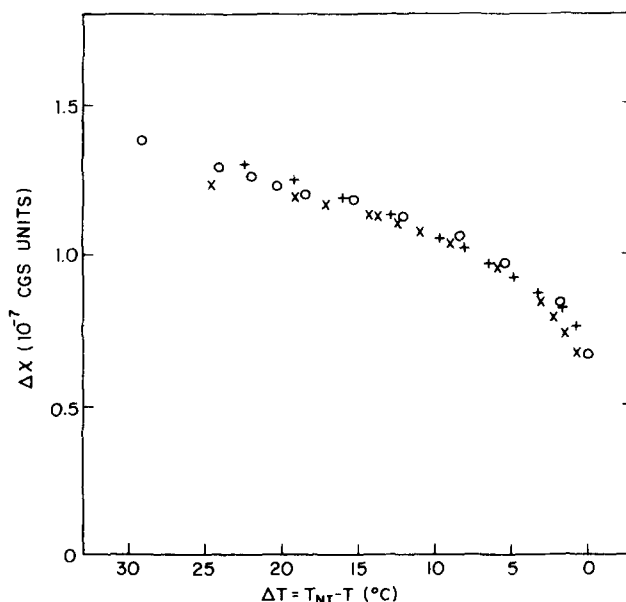
FIG. 11. Diamagnetic anisotropy of MBBA [ \circ : from G. Sigaud and H. Gasparoux, J. Chim. Phys. 70, 699 (1973), T_{NI}=46.0^\circ\text{C} ; \times : from I. Haller, J. Chem. Phys. 57, 1400 (1972), T_{NI}=41.3-45.7^\circ\text{C} ; + : from Ref. 49, T_{NI}=45.75^\circ\text{C} ].
