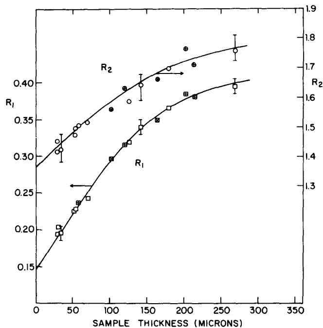
FIG. 7. Thickness dependence of measured depolarization ratios R_1 (squares) and R_2 (circles) of the cyano stretching band from samples of 20% BBCA in MBBA at 27.0 ^{\circ}\text{C} below transition. Data points with + and x are respectively those with static magnetic field of 5.6 and 0.9 kG along the direction of rubbing. T_{NI} ranges from 54.5 to 56.5 ^{\circ}\text{C} .
