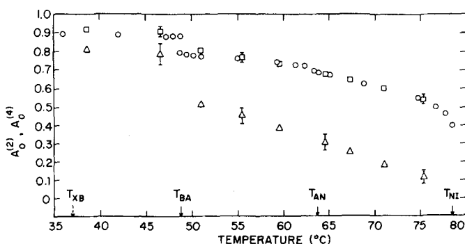
FIG. 21. Order parameters A_0^{(2)} (squares) and A_0^{(4)} (triangles) calculated from Raman measurements of the 1597 \text{cm}^{-1} band. Circles are relative values obtained from the optical dielectric anisotropy measurements.
