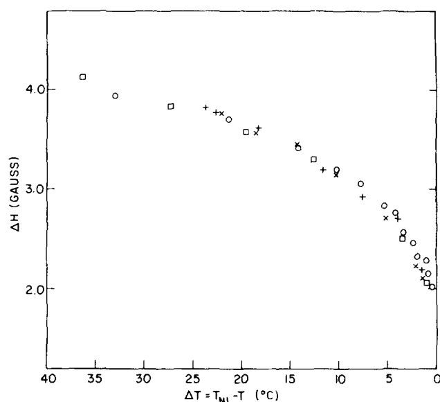
FIG. 10. Proton NMR splittings of MBBA [ \circ : T_{NI}=45.0^\circ\text{C} , from P. Papon and J.-P. Lepesant, Chem. Phys. Lett. 12, 331 (1971); + : T_{NI}=46.64^\circ\text{C} ; \times : T_{NI}=42.70^\circ\text{C} ] and 20% BBBA in MBBA [ \square : T_{NI}=55.84^\circ\text{C} ].
