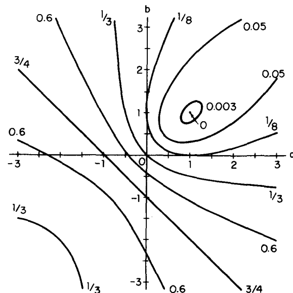
FIG. 23. Contours of constant R_{\text{iso}} in the (a, b) plane.
