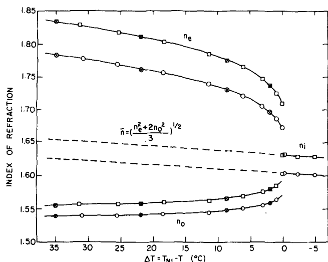
FIG. 8. Indices of refraction of 20% BBBA in MBBA. Squares are measured at 5145 Å, and circles at 6328 Å. ( T_{NI}=55.25^\circ\text{C} for crossed data points, T_{NI}=53.78^\circ\text{C} for open points).
