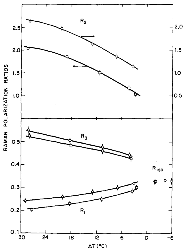
FIG. 17. Raman depolarization ratios R_1 , R_2 , R_3 , and R_{iso} of the 1597\text{ cm}^{-1} band for samples of 20% BBBA in MBBA. Circles: 76.1\text{ }\mu ; squares: 51.5\text{ }\mu thick.
