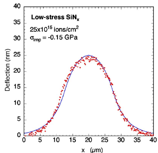
FIG. 9. (Color online) Experimental deflection of a low-stress silicon nitride membrane for the case where a circular region with a 15 \mu\text{m} diameter was implanted with 25 \times 10^{15} Ga + ions/cm 2 . The solid line is the shape predicted by the model.
