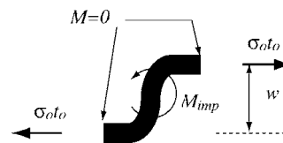
FIG. 11. Schematic illustration of the bending moments applied to a section of a membrane with a large \beta value. Cross sections of horizontal segments of the membrane do not have any resultant bending moment.
