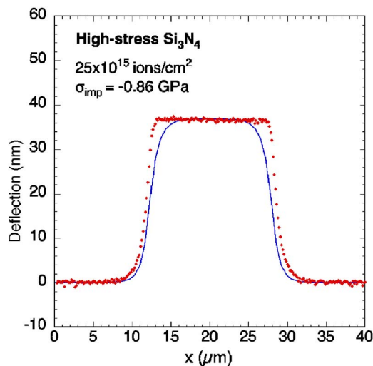
FIG. 10. (Color online) Experimental deflection of a high-stress silicon nitride membrane for the case where a circular region with a 15\ \mu\text{m} diameter was implanted with 25 \times 10^{15}\ \text{Ga}^+ ions/ \text{cm}^2 . The solid line is the shape predicted by the model.
